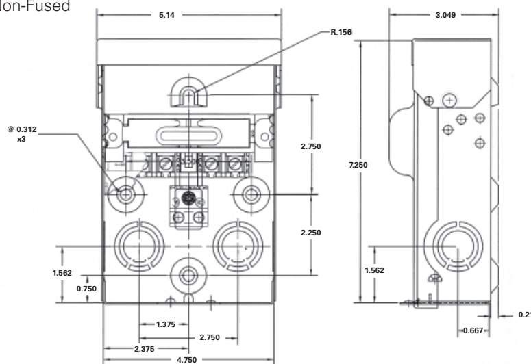
Removable Door
