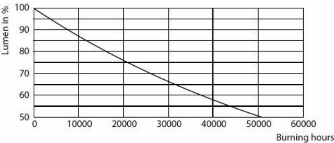
Lumen Maintenance Diagram - 8.5PAR30S/COR/927/F40/D/P/ULW/T20 6/1FB
