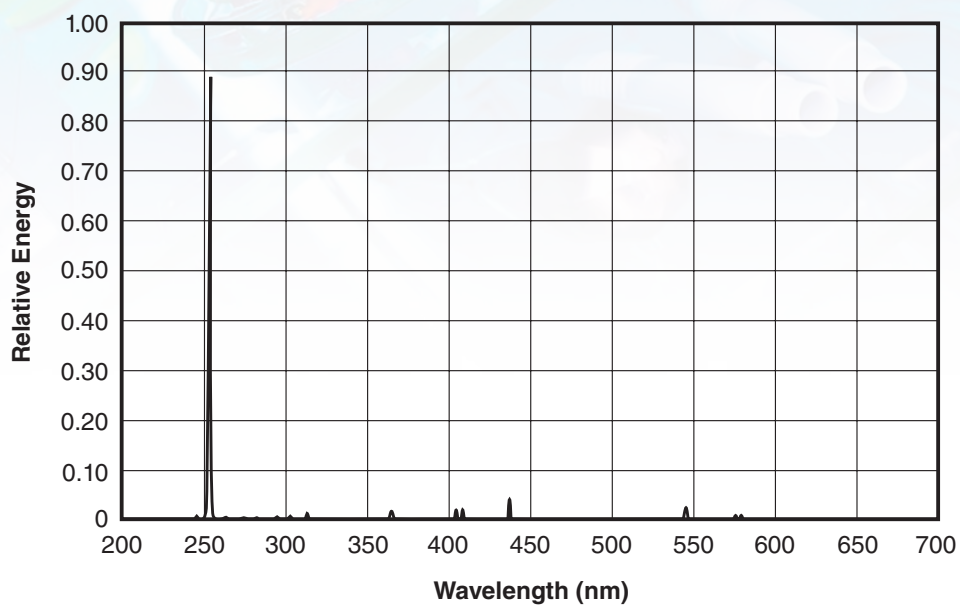
SPECTRAL DISTRIBUTION ULTRAVIOLET LAMP - 253.7nm
