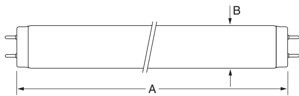
T8 and T10 Medium Bi-Pin G13 Base
