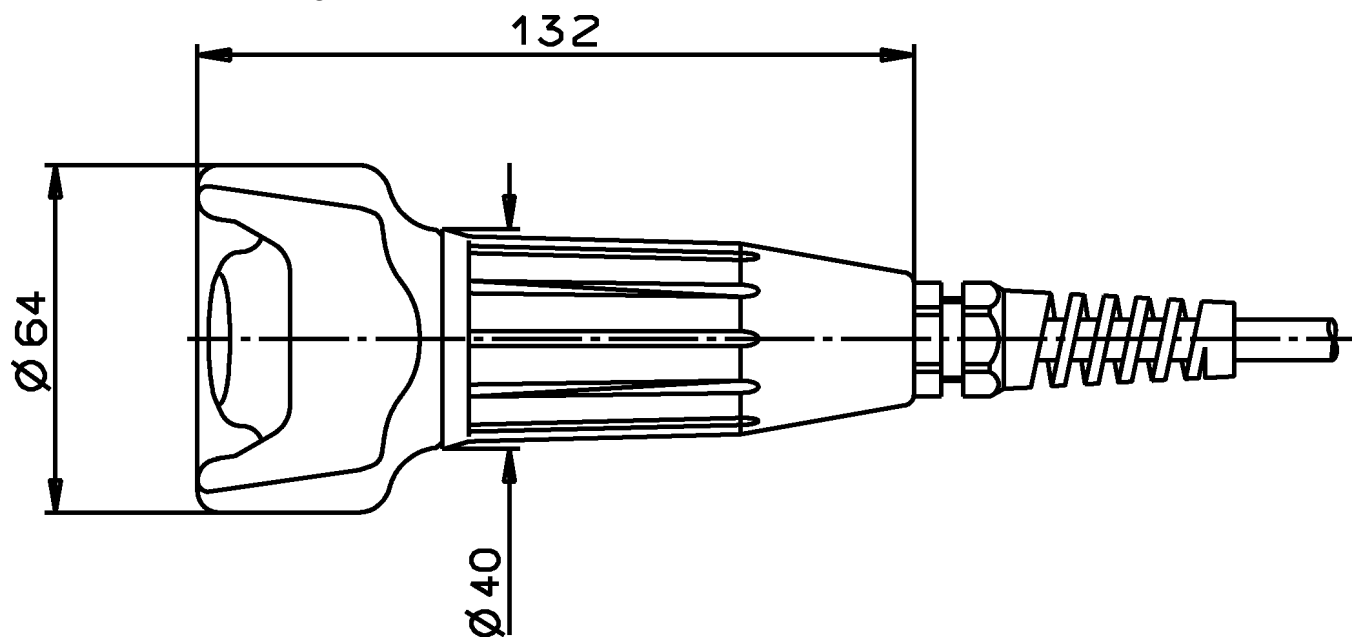
Dimensional drawings
