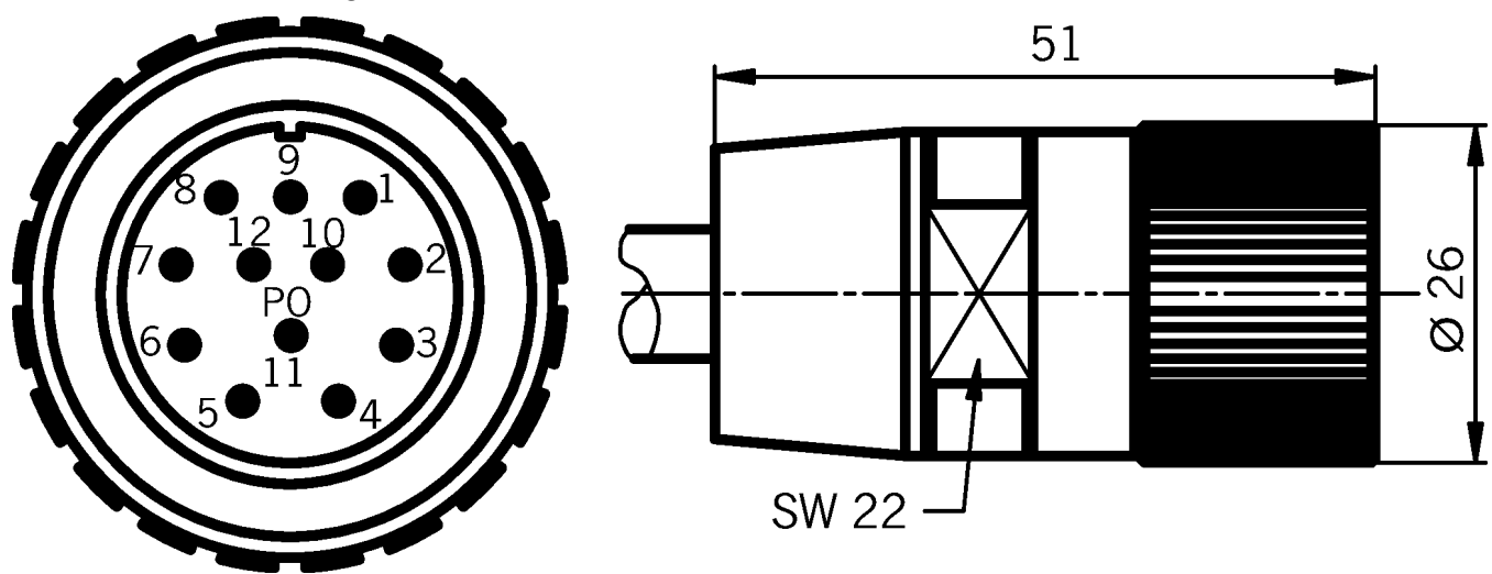
Dimensional drawings
