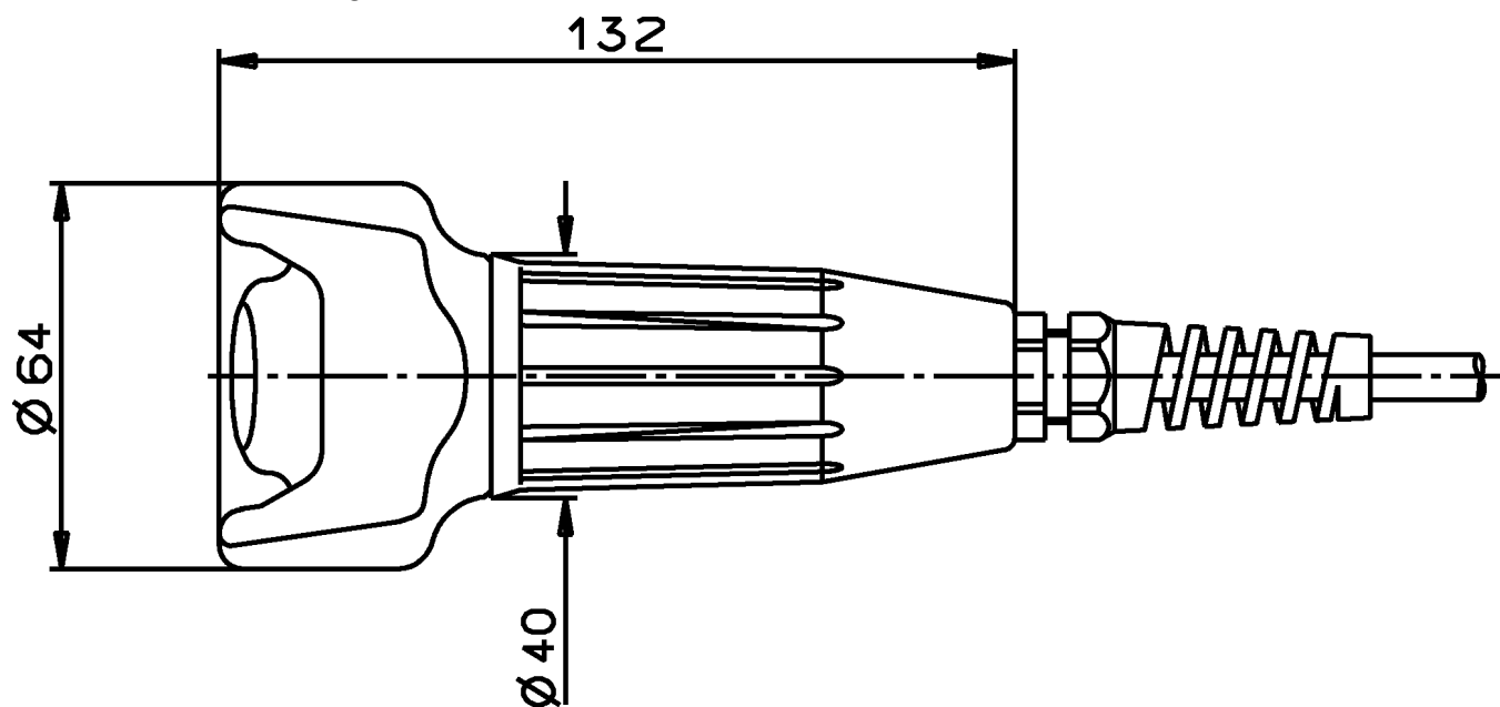
Dimensional drawings
