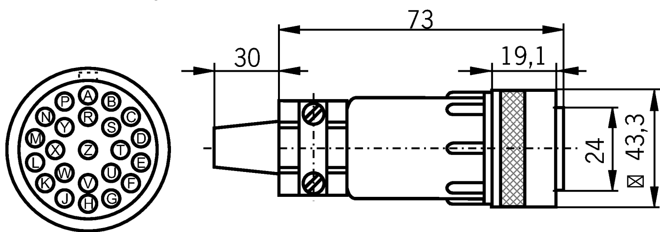
Dimensional drawings
