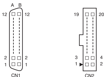
Connector Pin Diagram (from Connector Mating Side)
