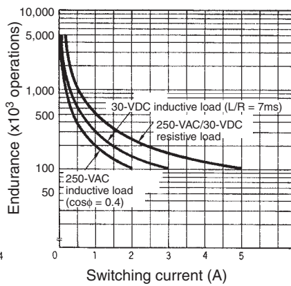
G2R-2-S (S)
