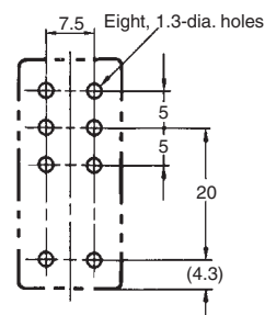
Mounting Holes (Bottom View)
