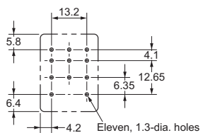
Eleven, 1.3-dia. holes
