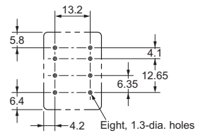
Eight, 1.3-dia. holes
