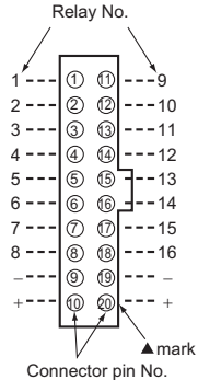
Connector Pin (male) Configuration View from engaged side
