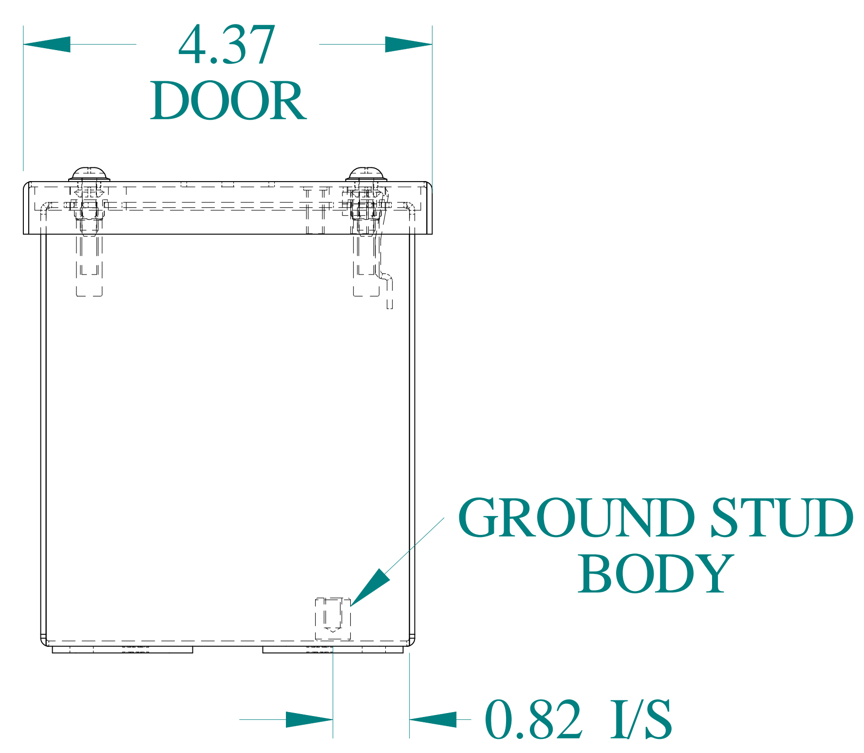
BOTTOM VIEW
