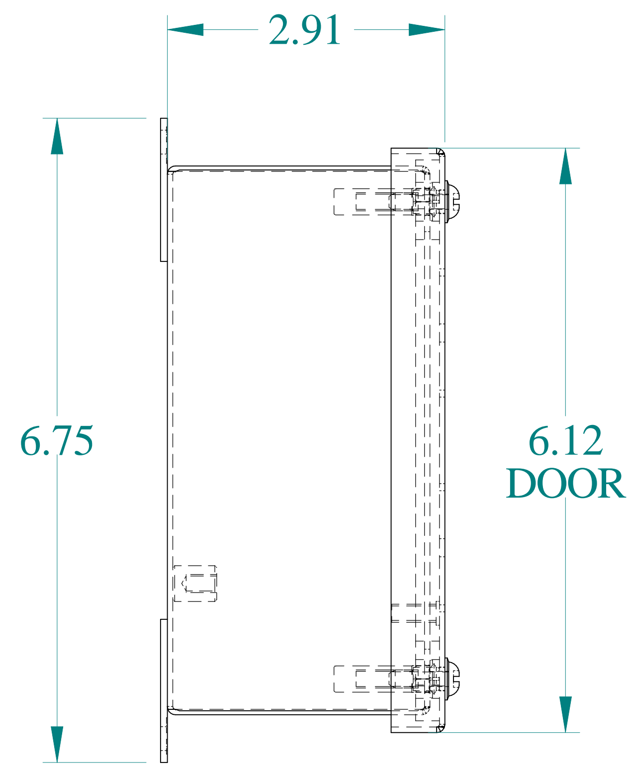
SIDE VIEW
