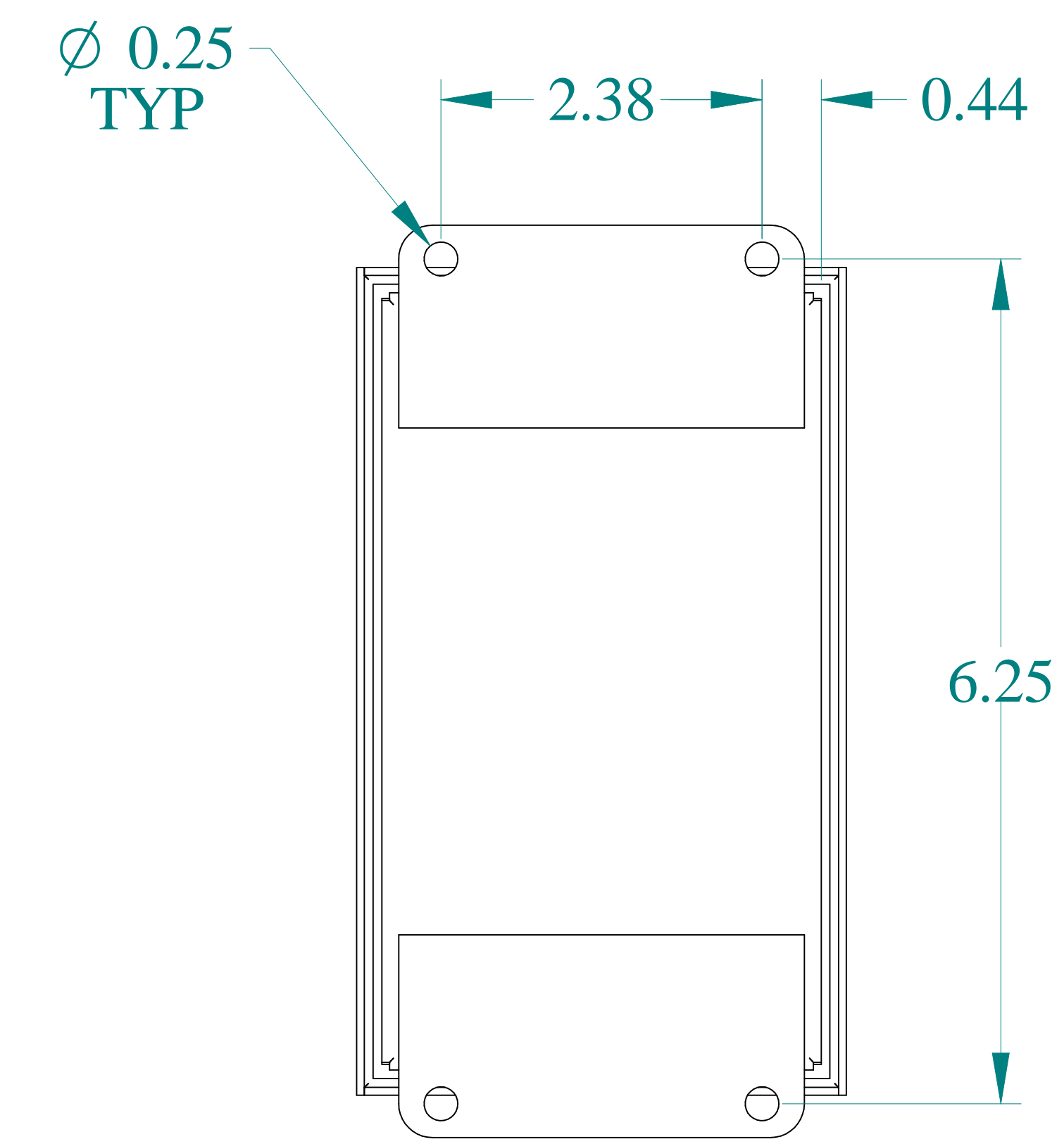
BACK VIEW
