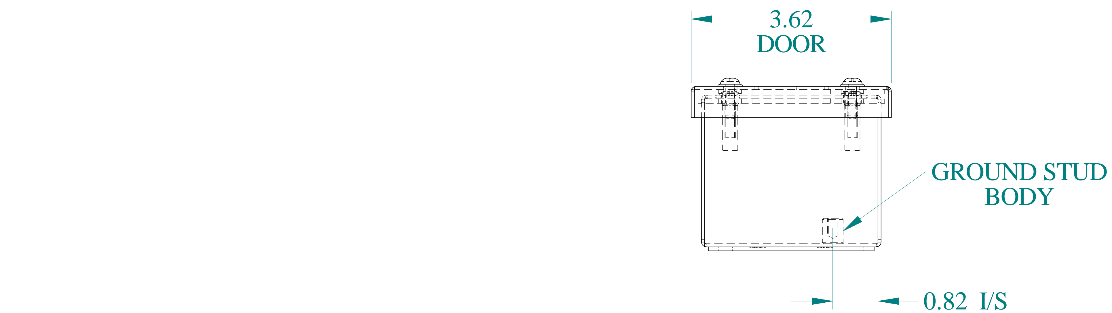
BOTTOM VIEW
