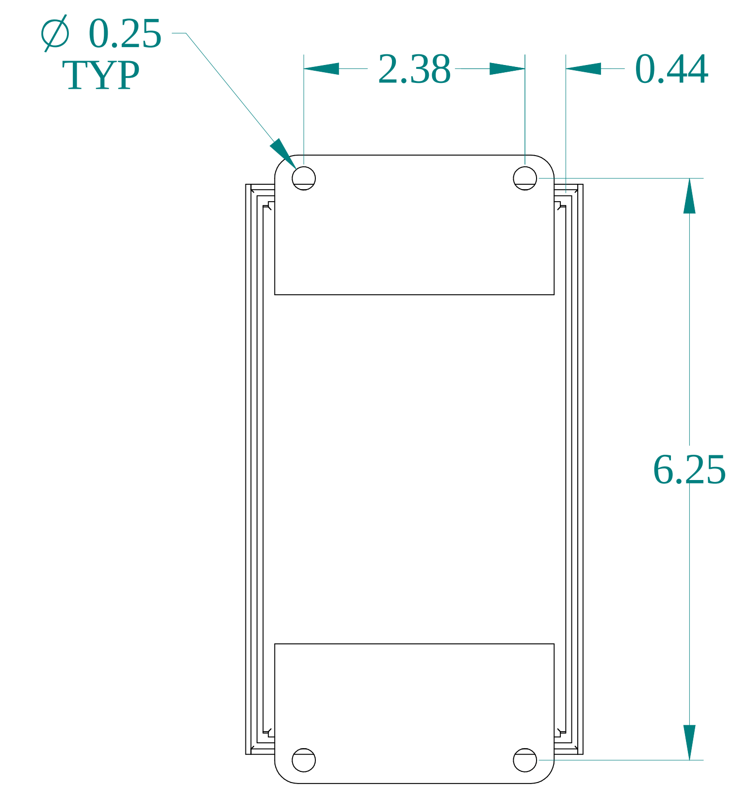
BACK VIEW
