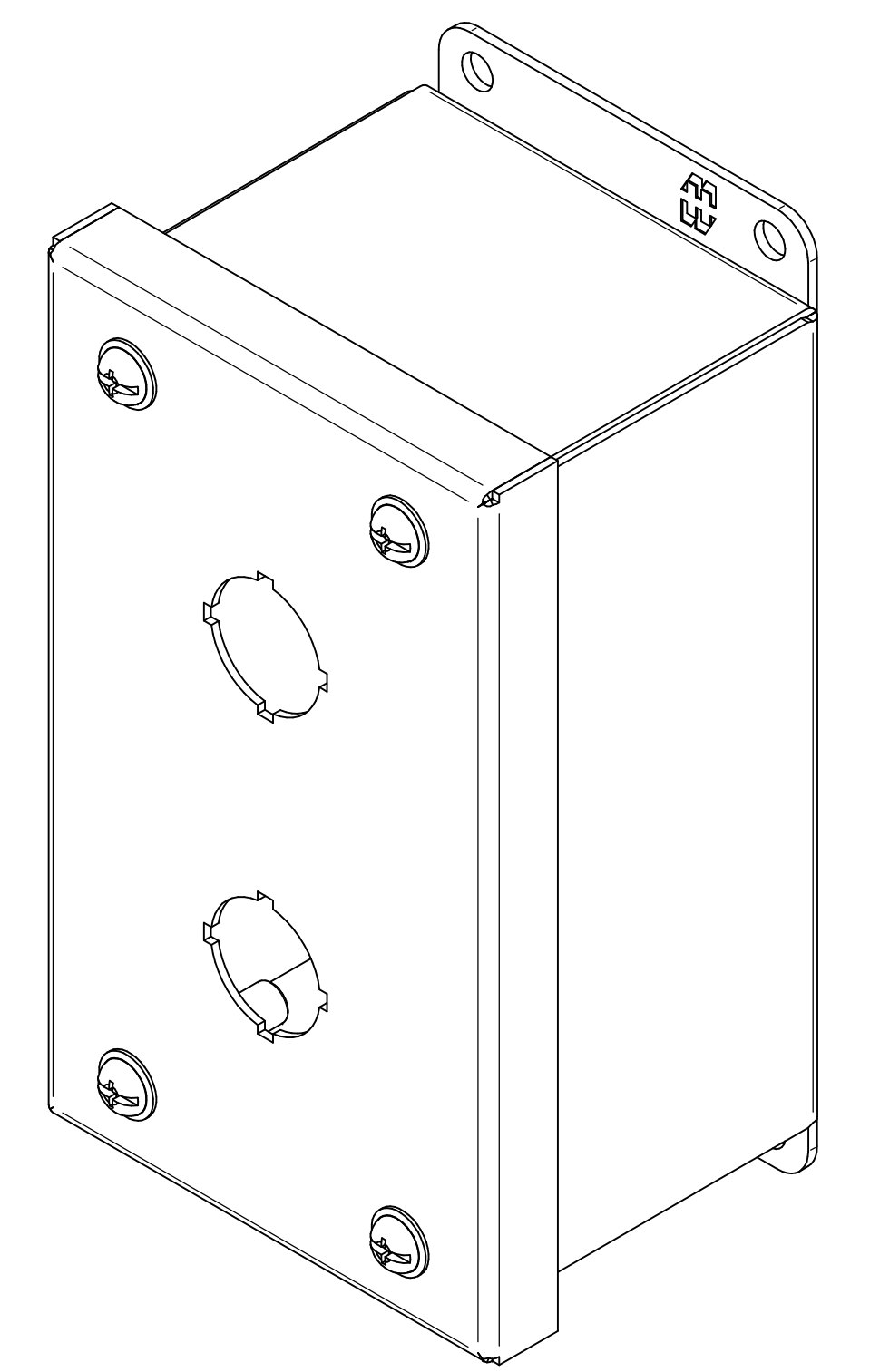
ISOMETRIC VIEWS
