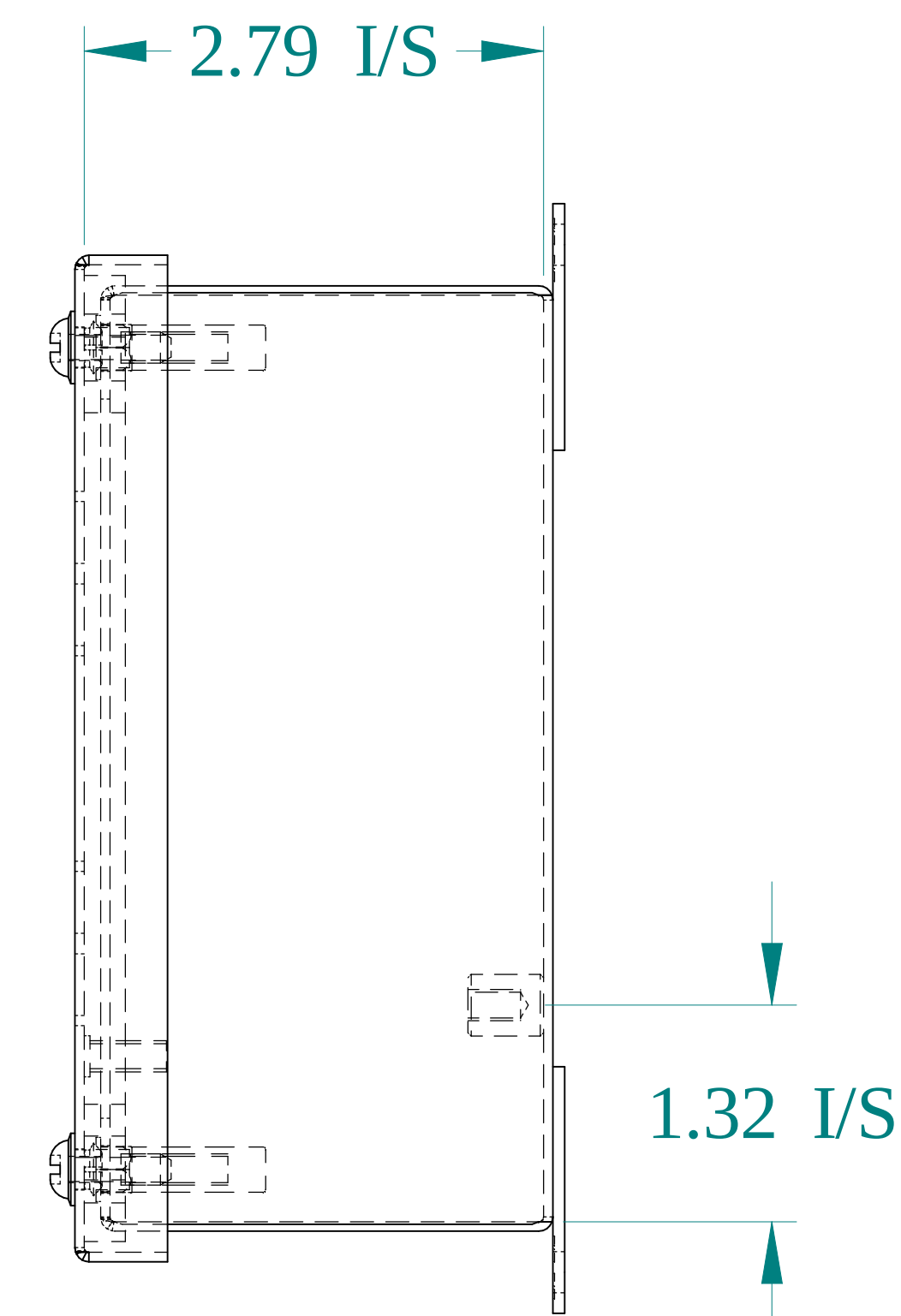
SIDE VIEW
