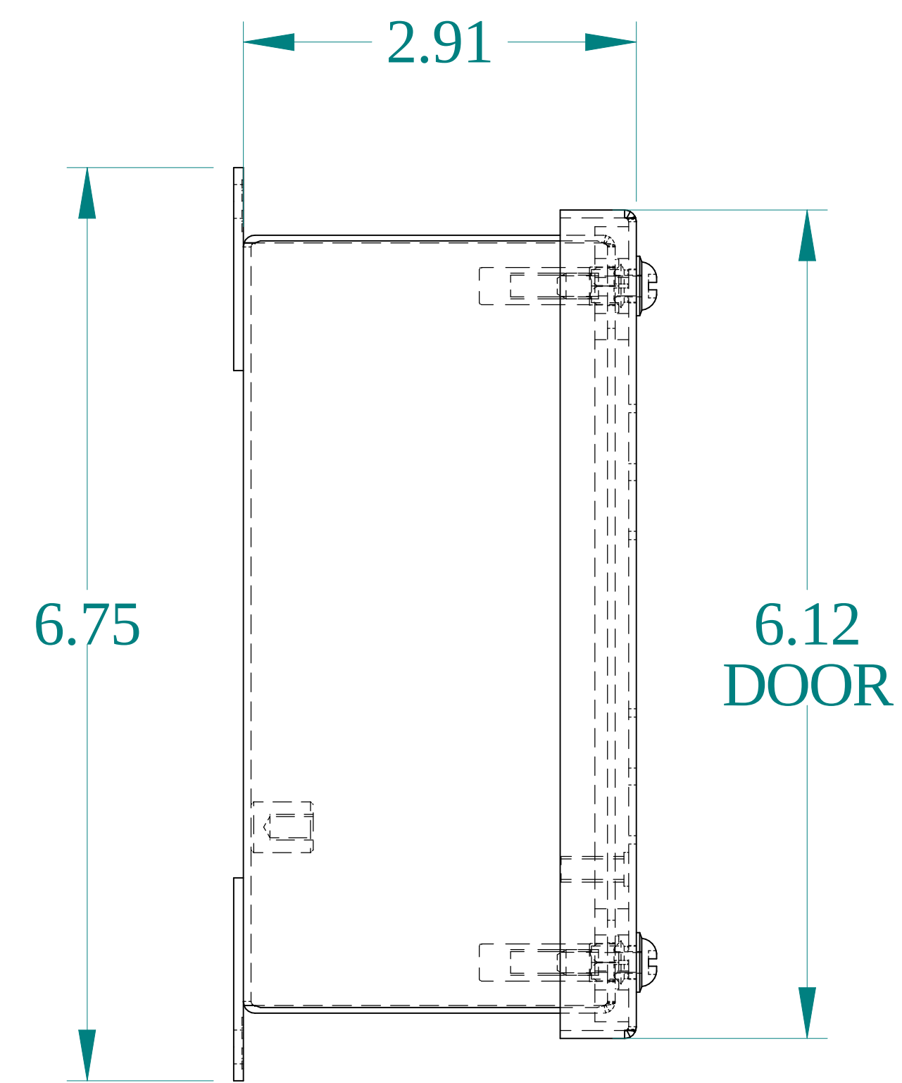
SIDE VIEW
