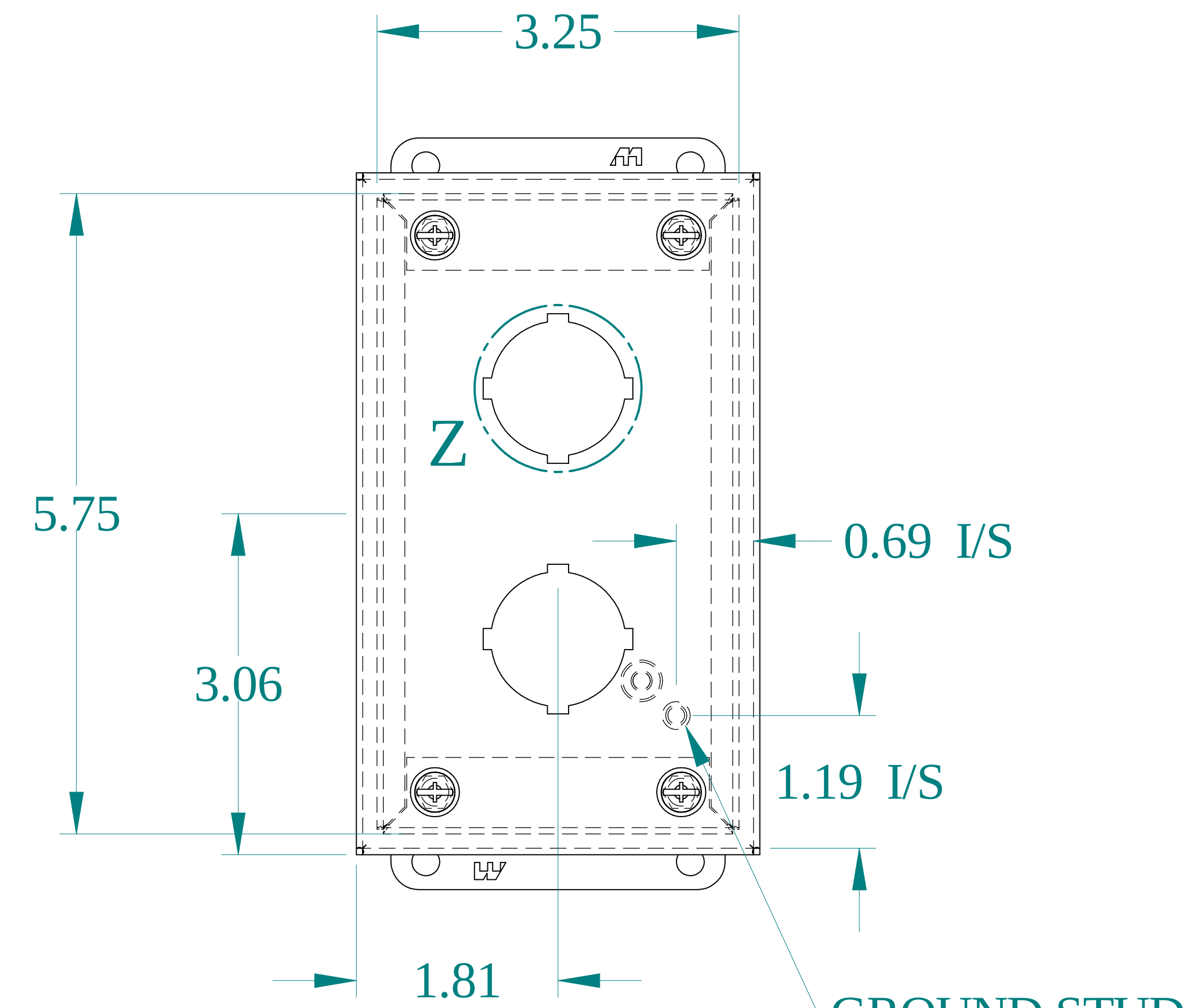
FRONT VIEW
