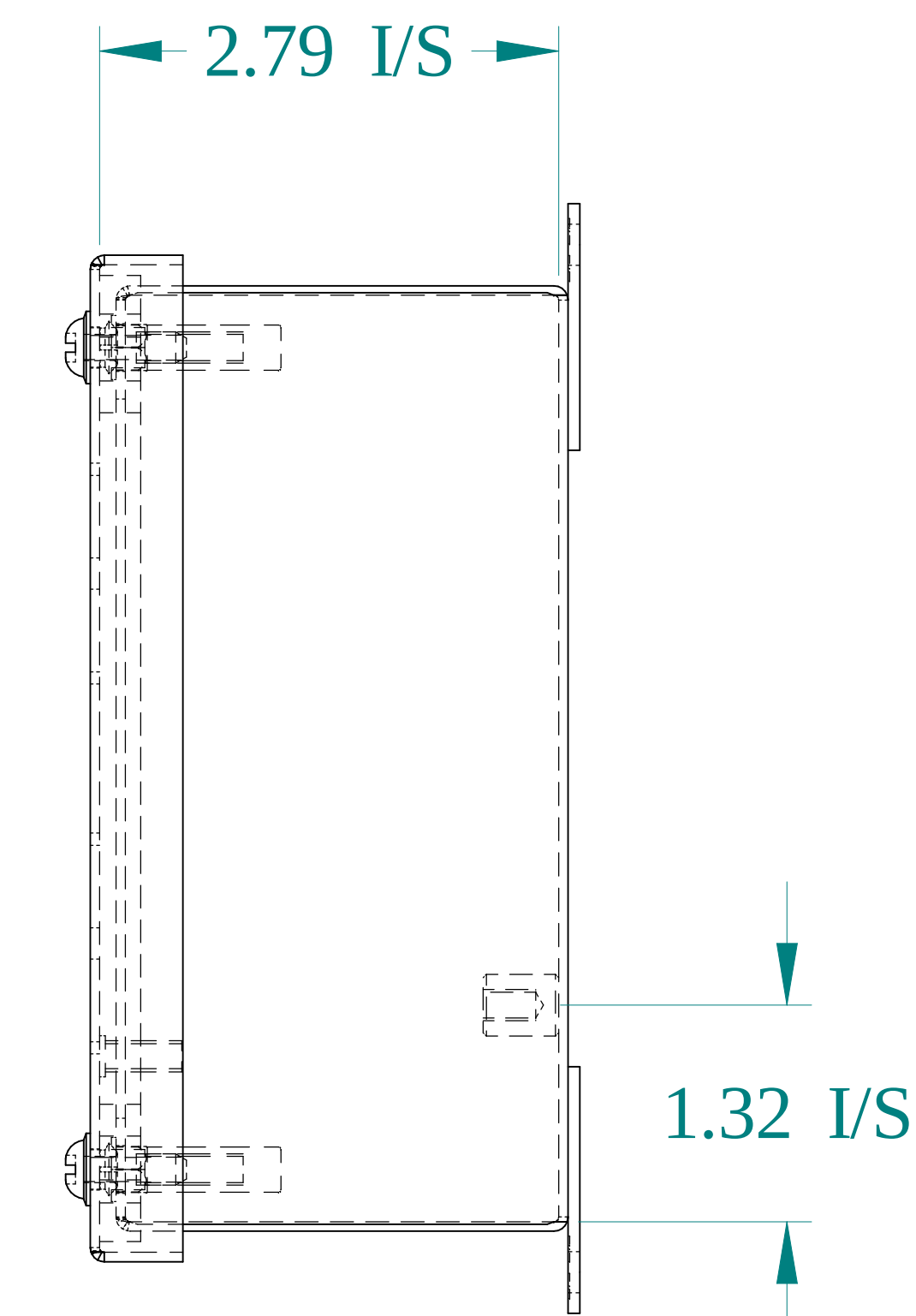
SIDE VIEW
