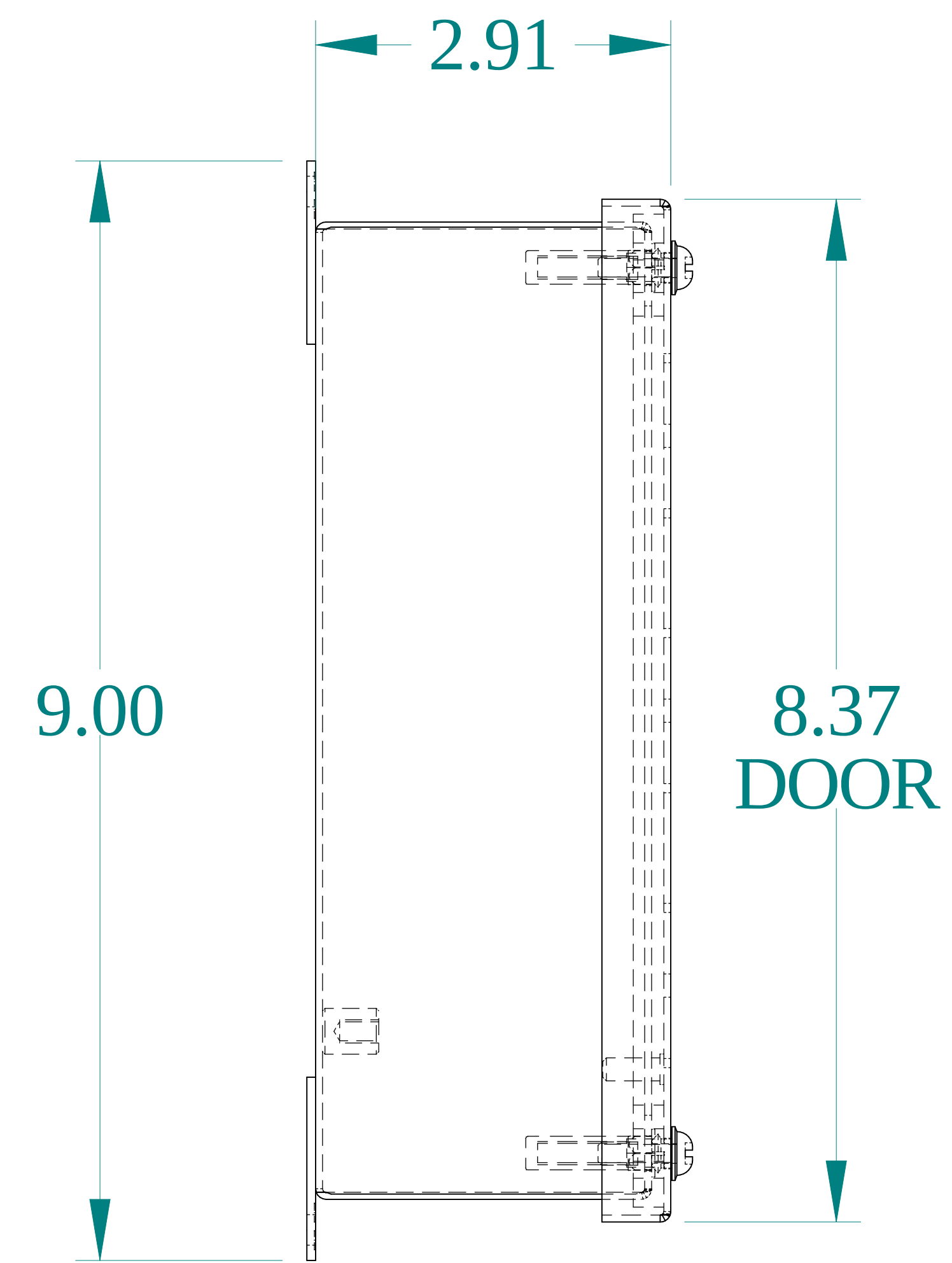
SIDE VIEW
