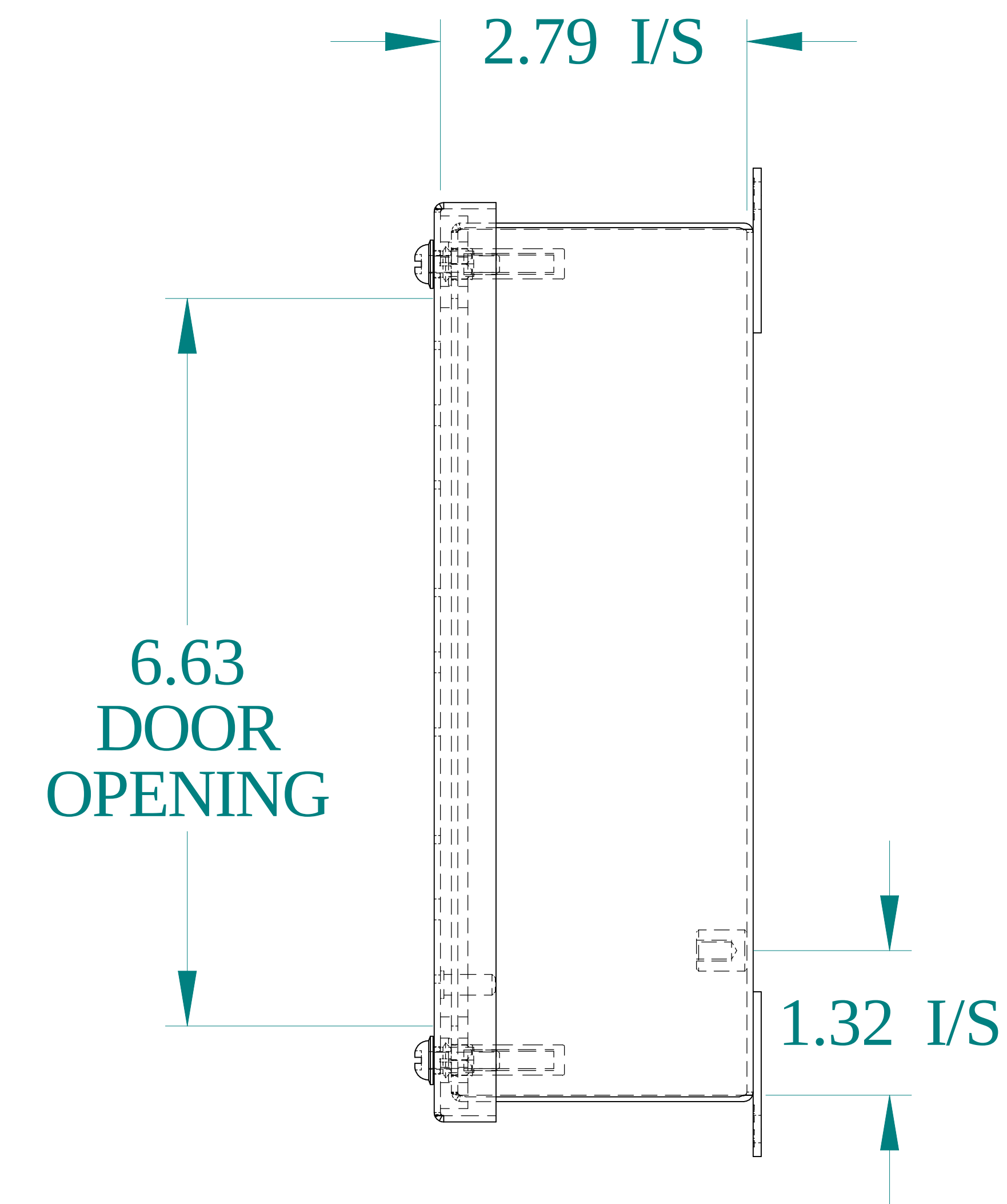
SIDE VIEW
