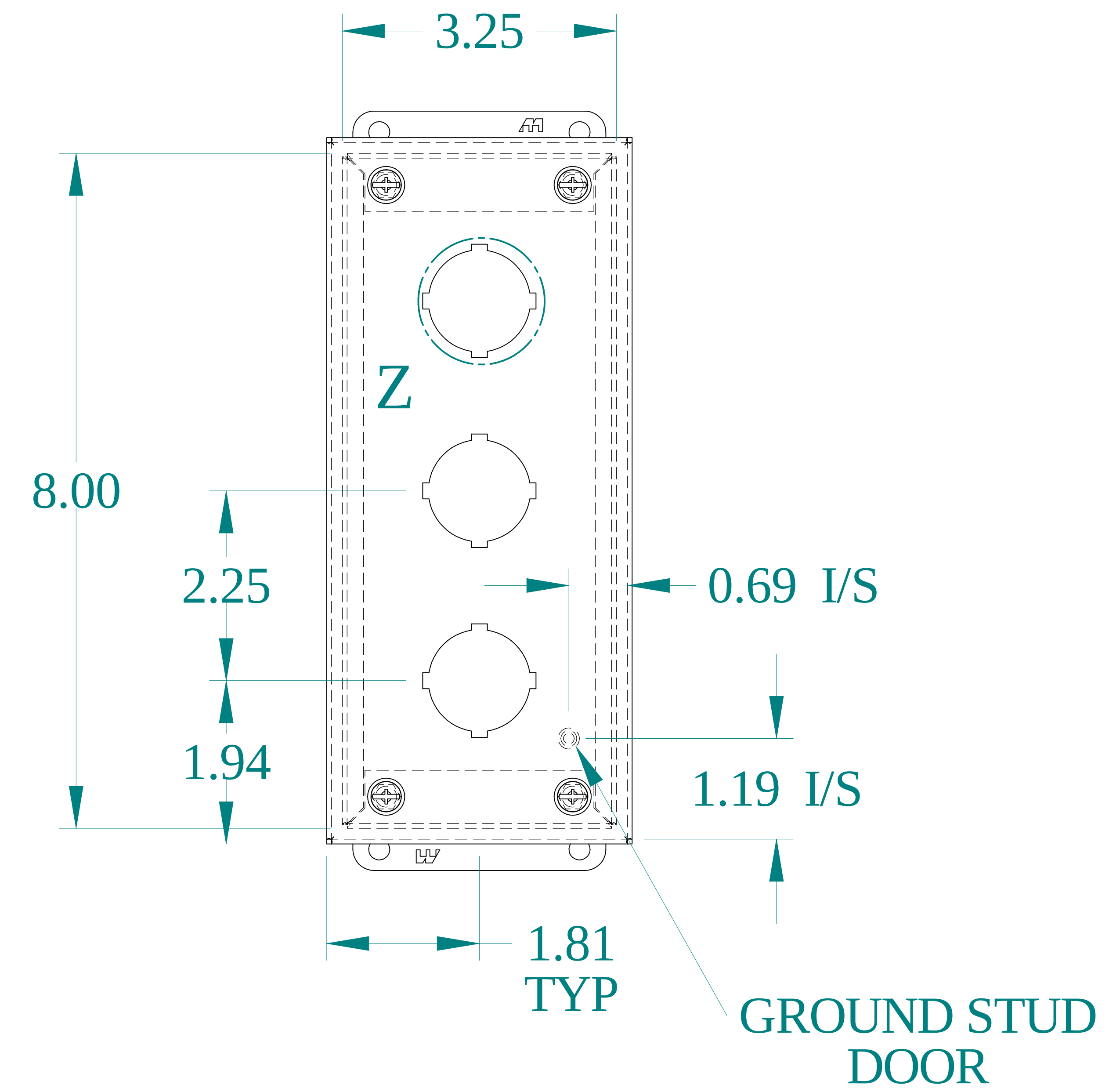
FRONT VIEW
