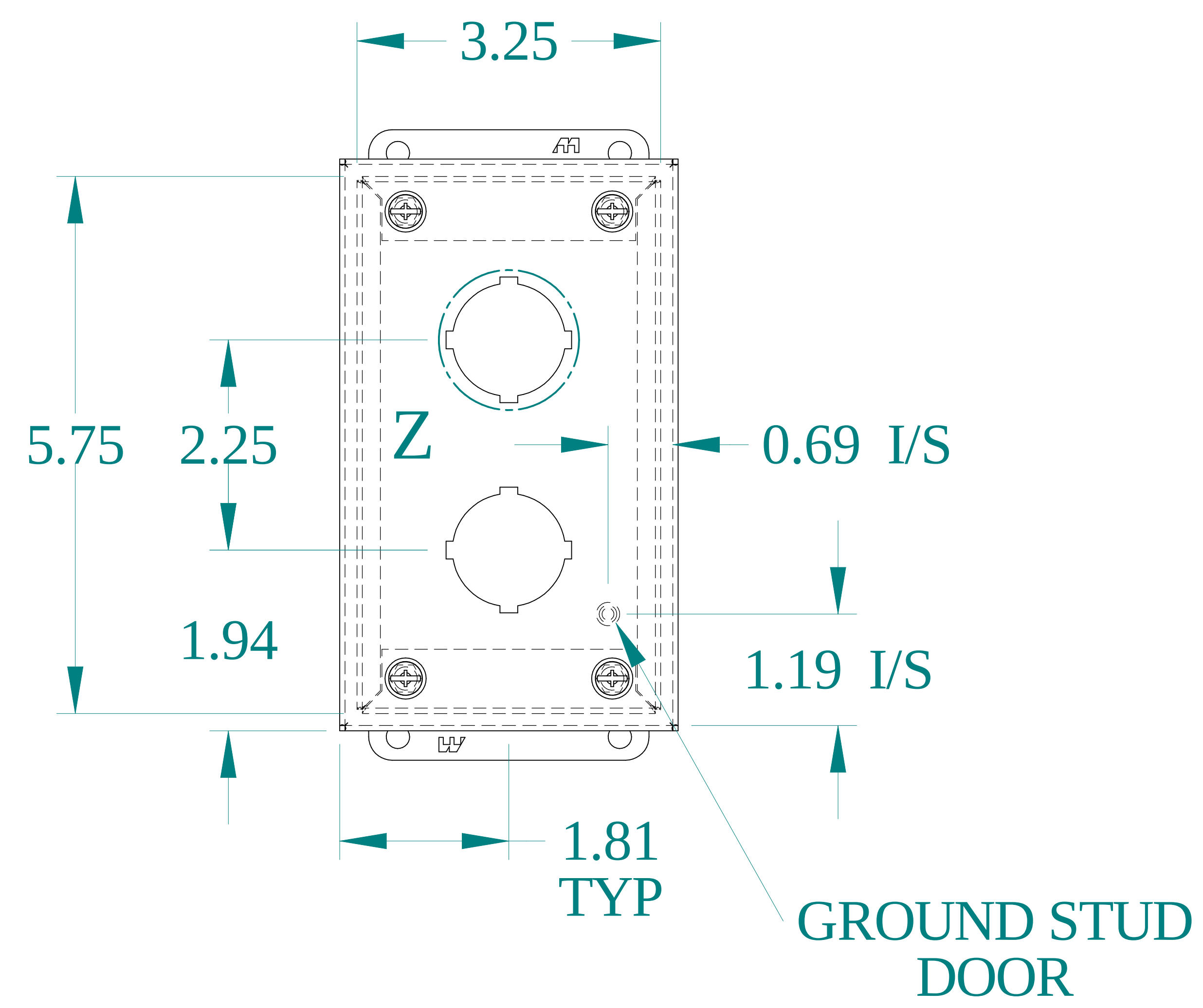
FRONT VIEW
