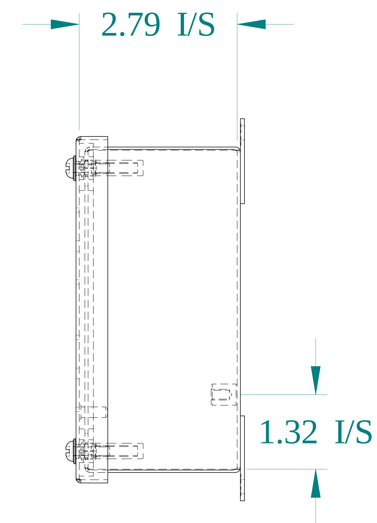
SIDE VIEW
