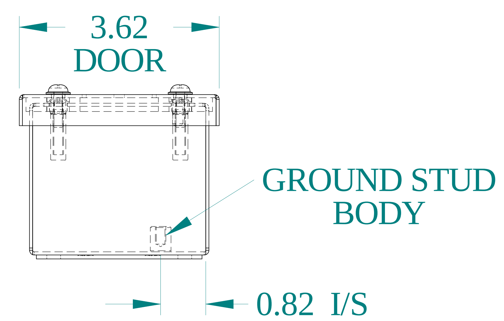
BOTTOM VIEW
