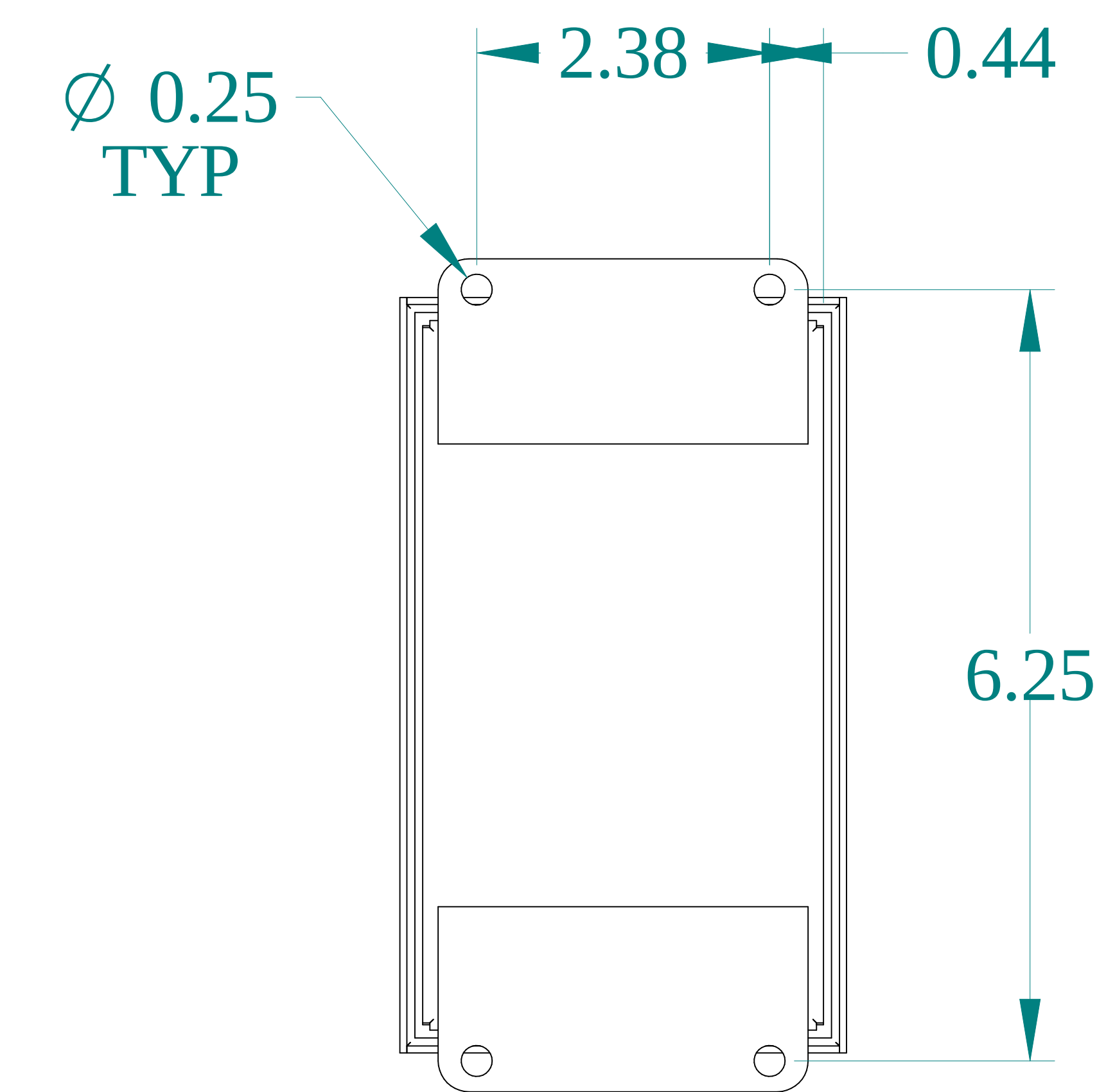
BACK VIEW
