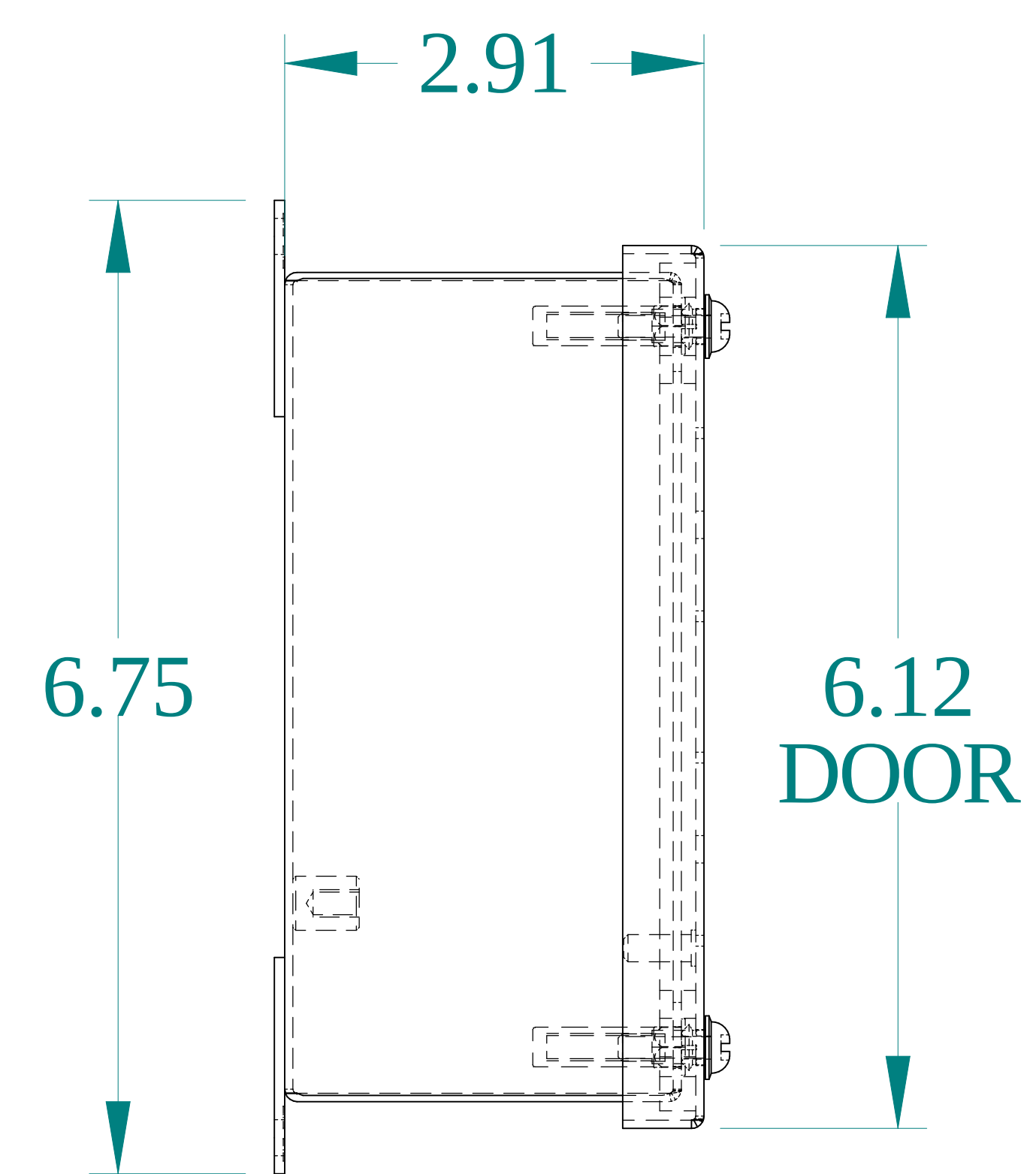
SIDE VIEW
