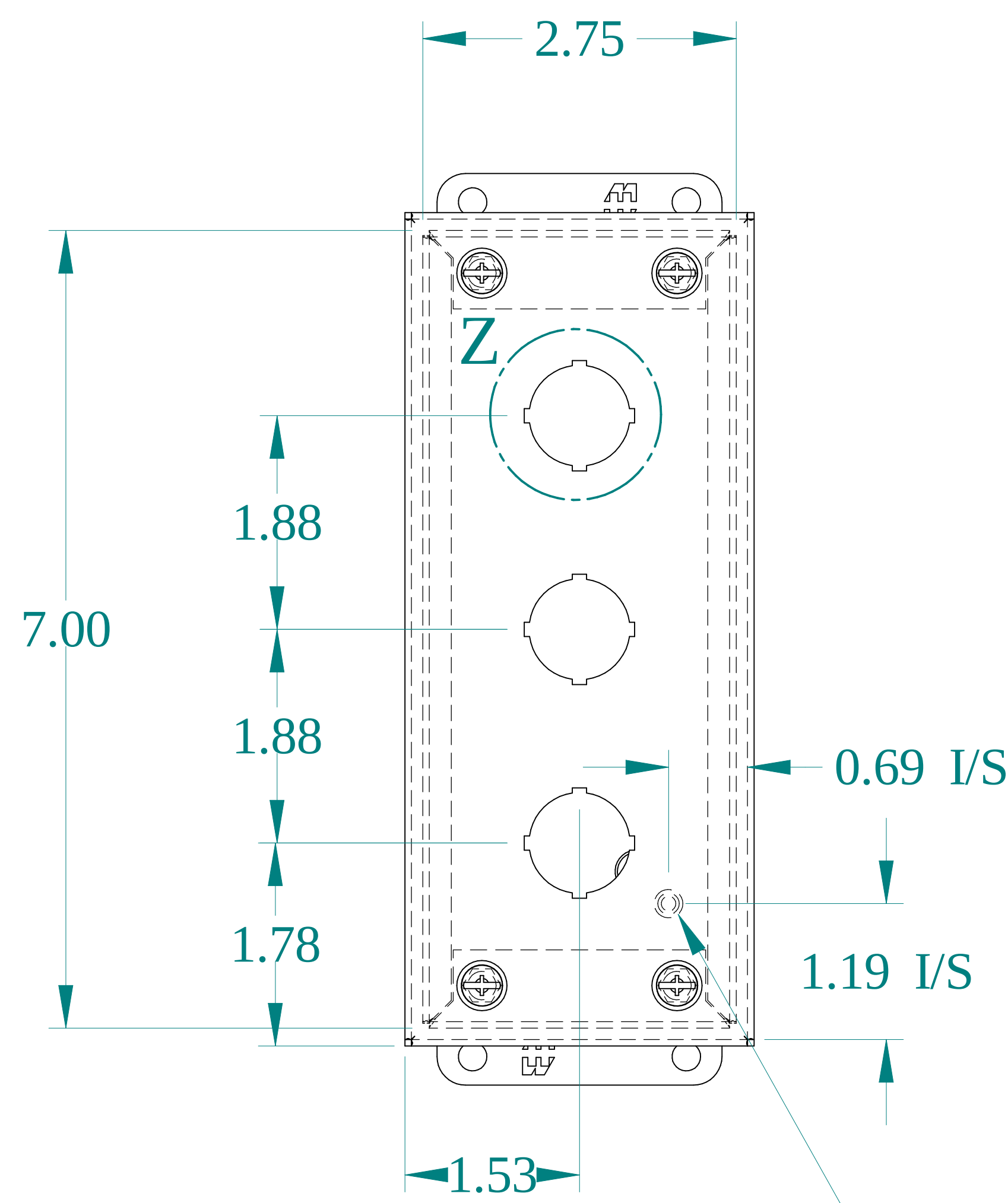
FRONT VIEW
