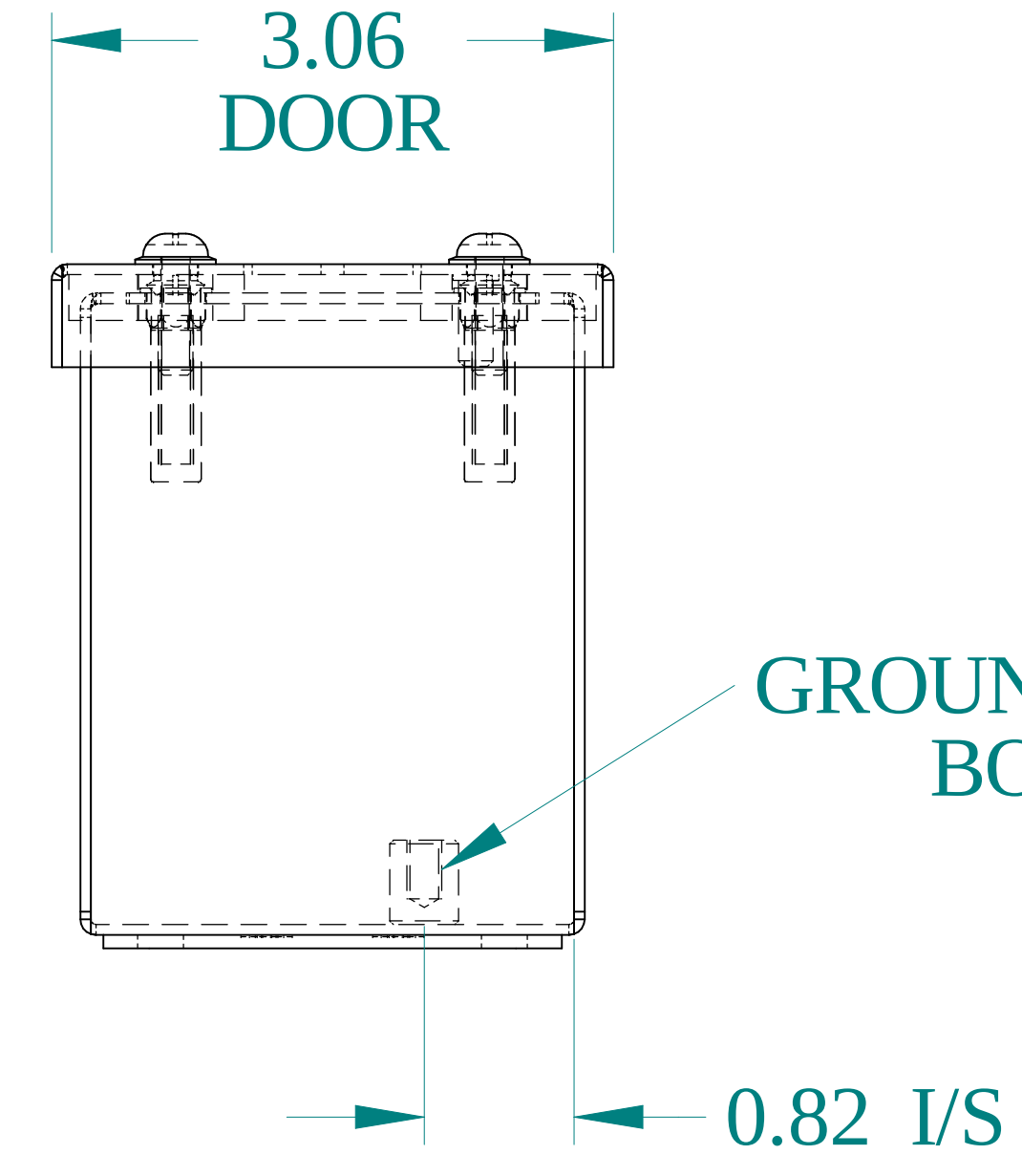
BOTTOM VIEW
