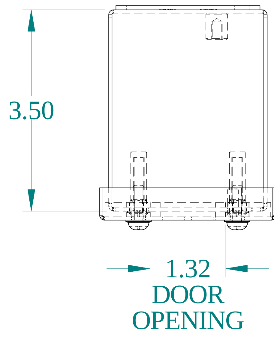
TOP VIEW
