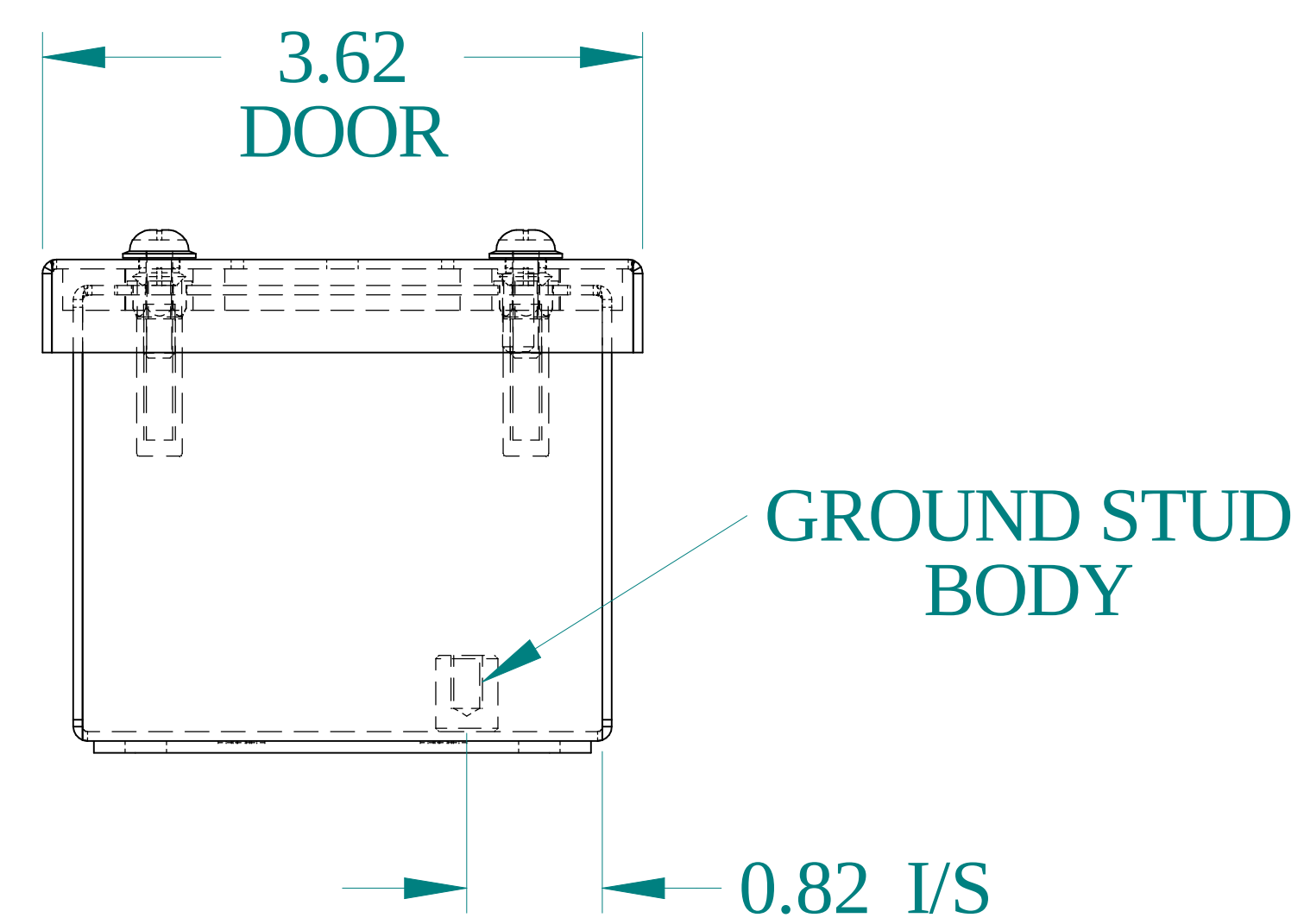
BOTTOM VIEW
