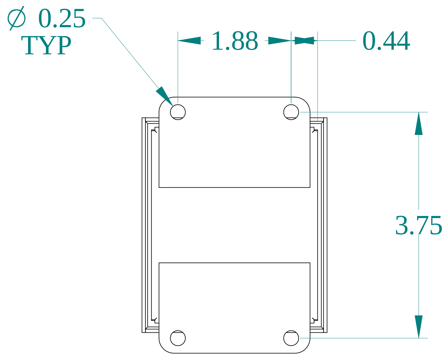
BACK VIEW
