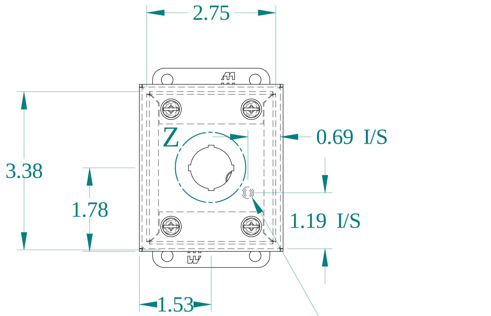
FRONT VIEW
