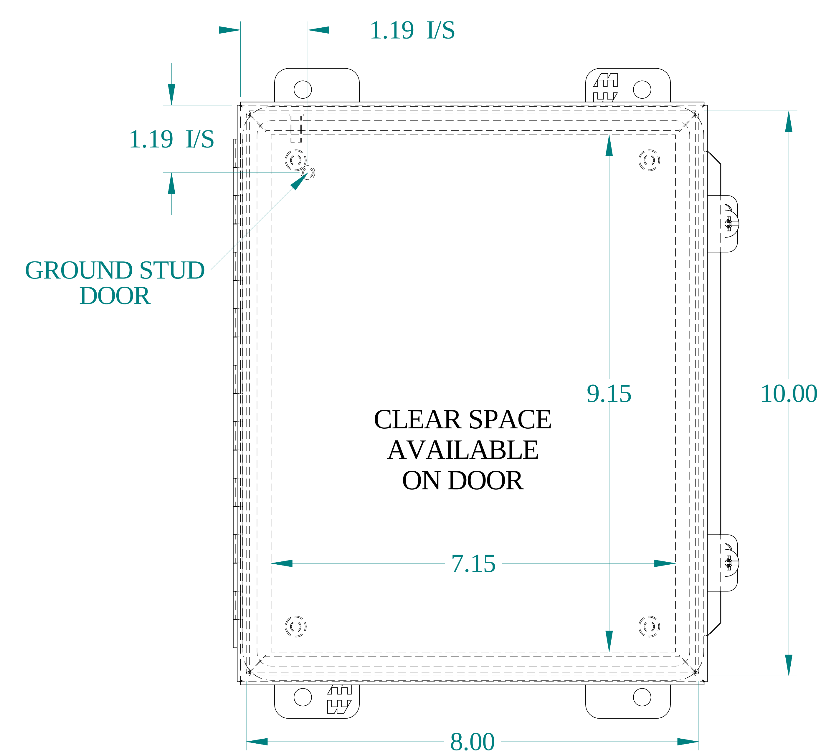
FRONT VIEW
