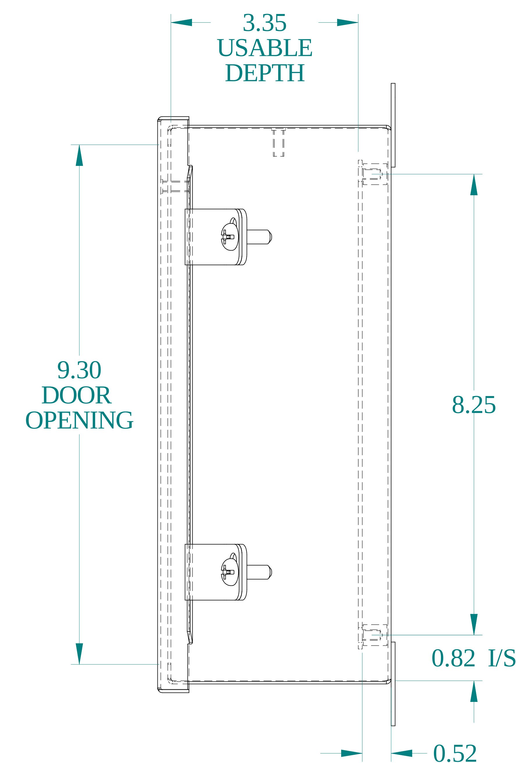
SIDE VIEW
