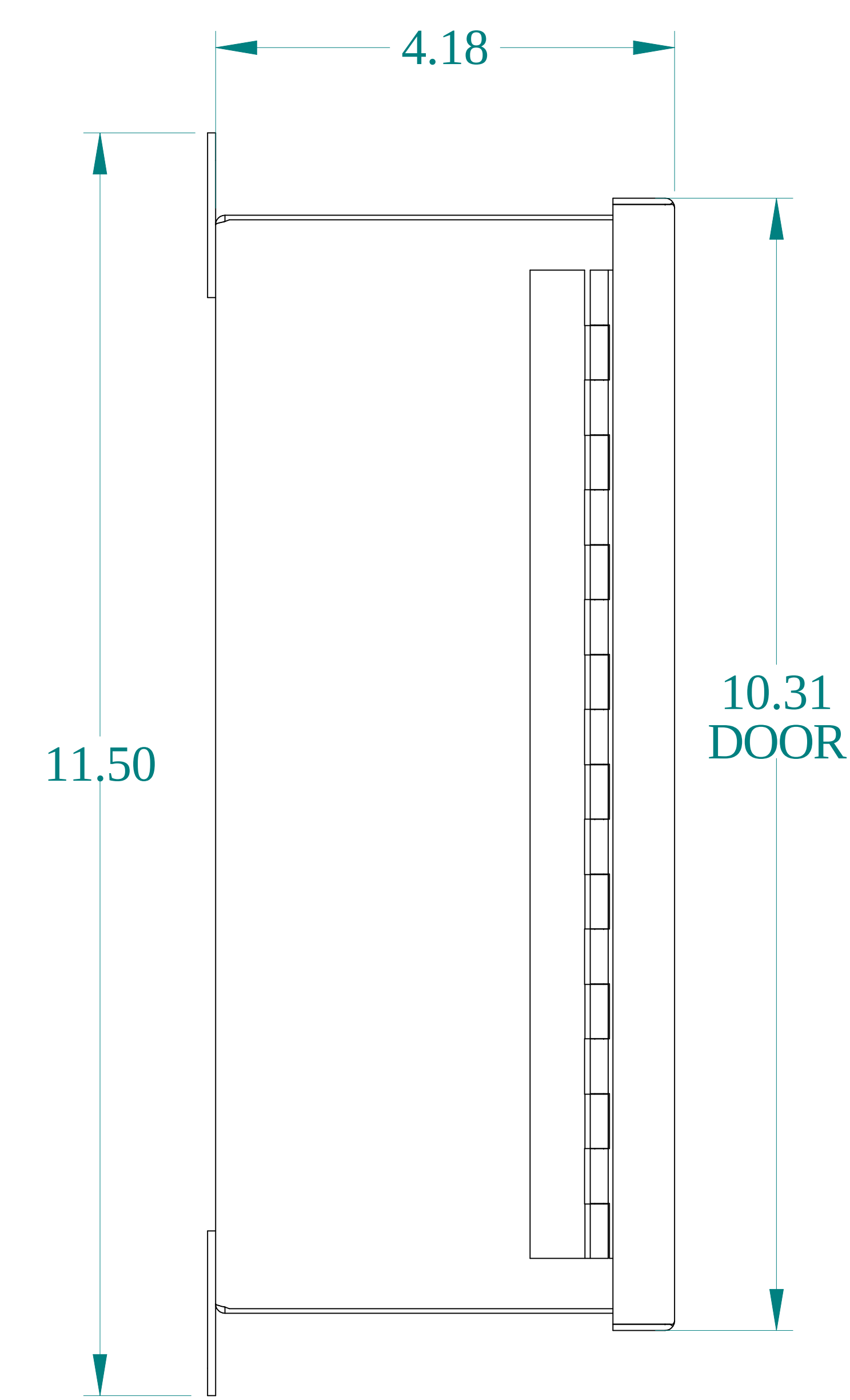
SIDE VIEW
