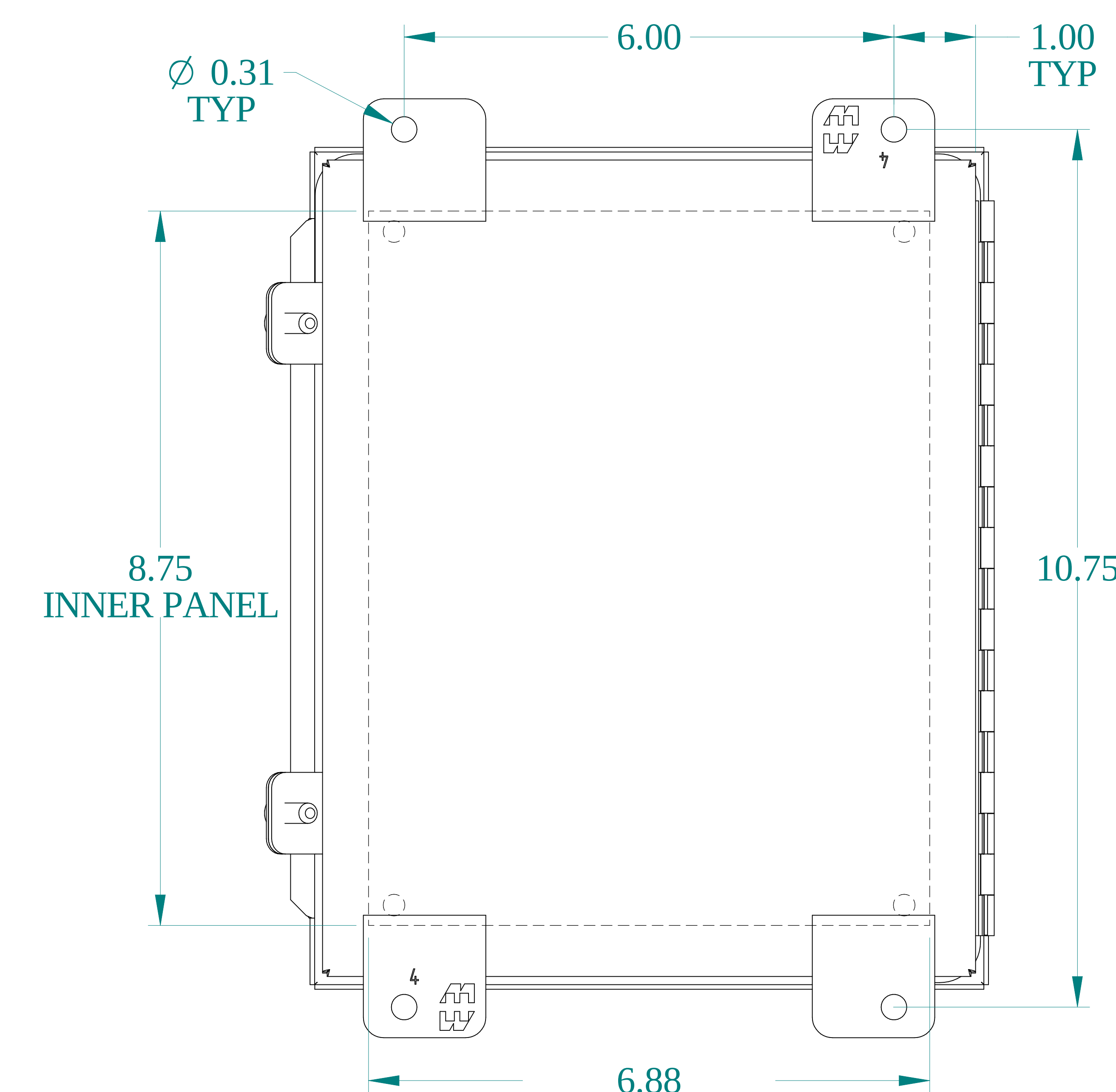
BACK VIEW
