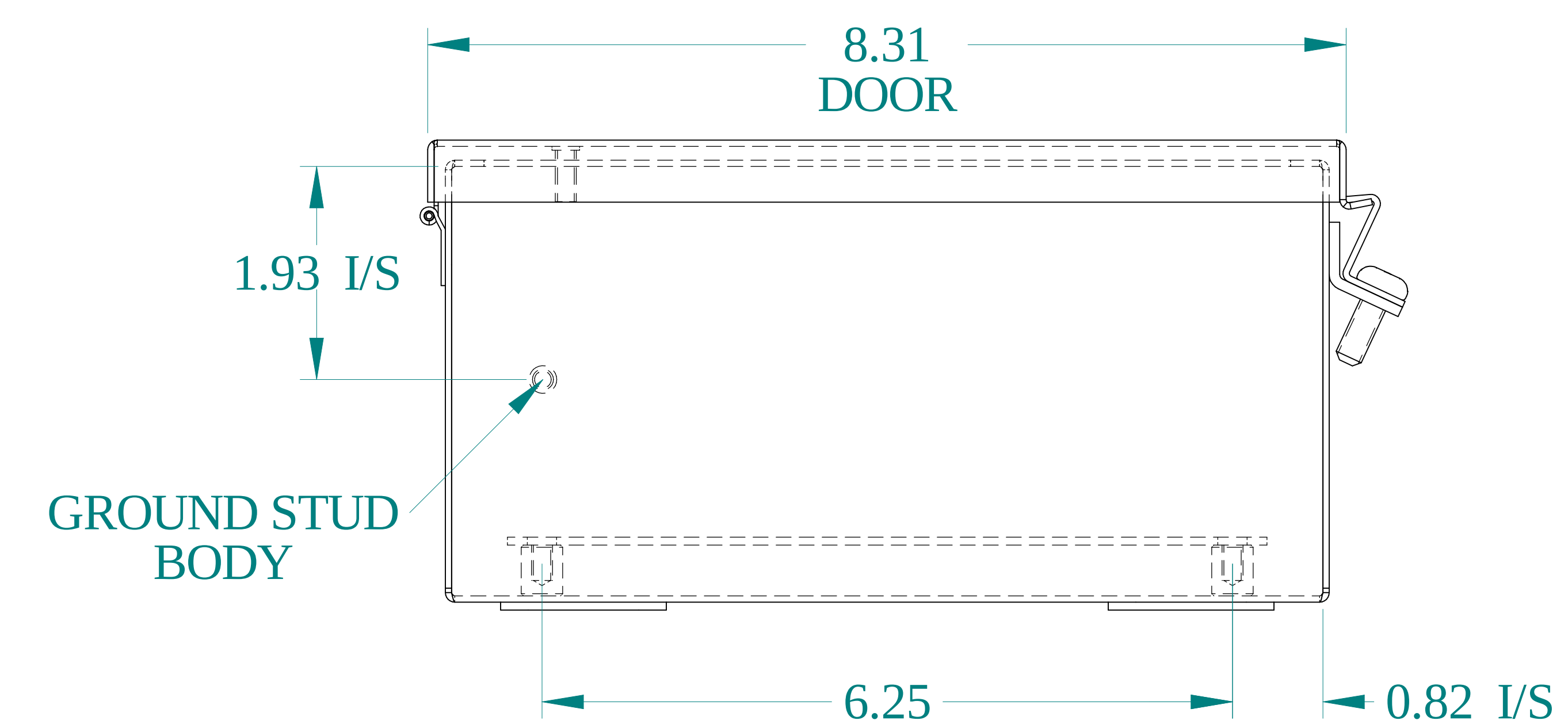
BOTTOM VIEW
