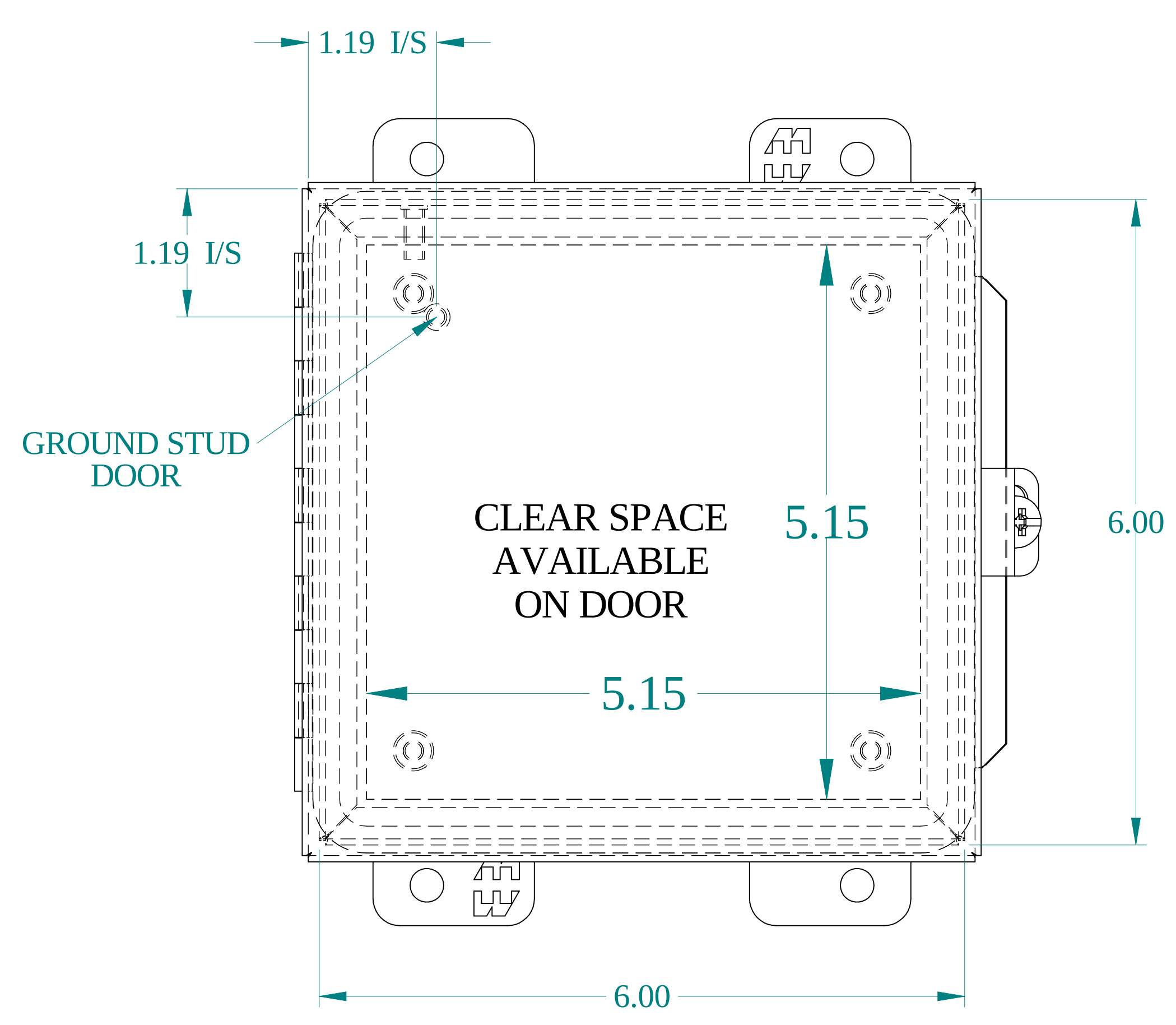
FRONT VIEW
