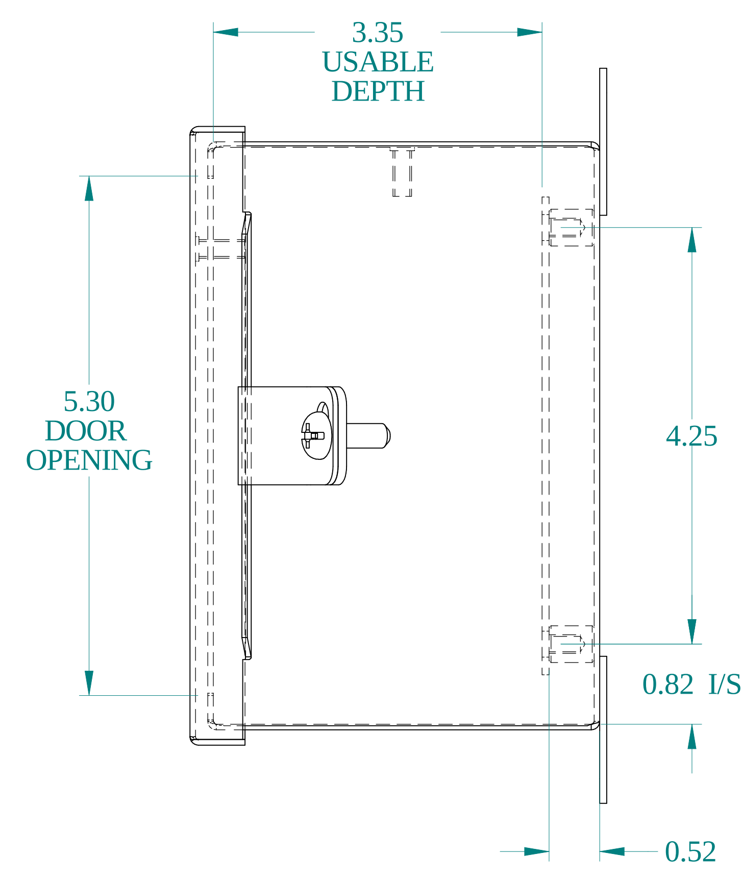
SIDE VIEW
