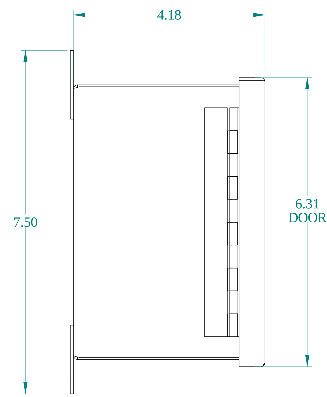
SIDE VIEW
