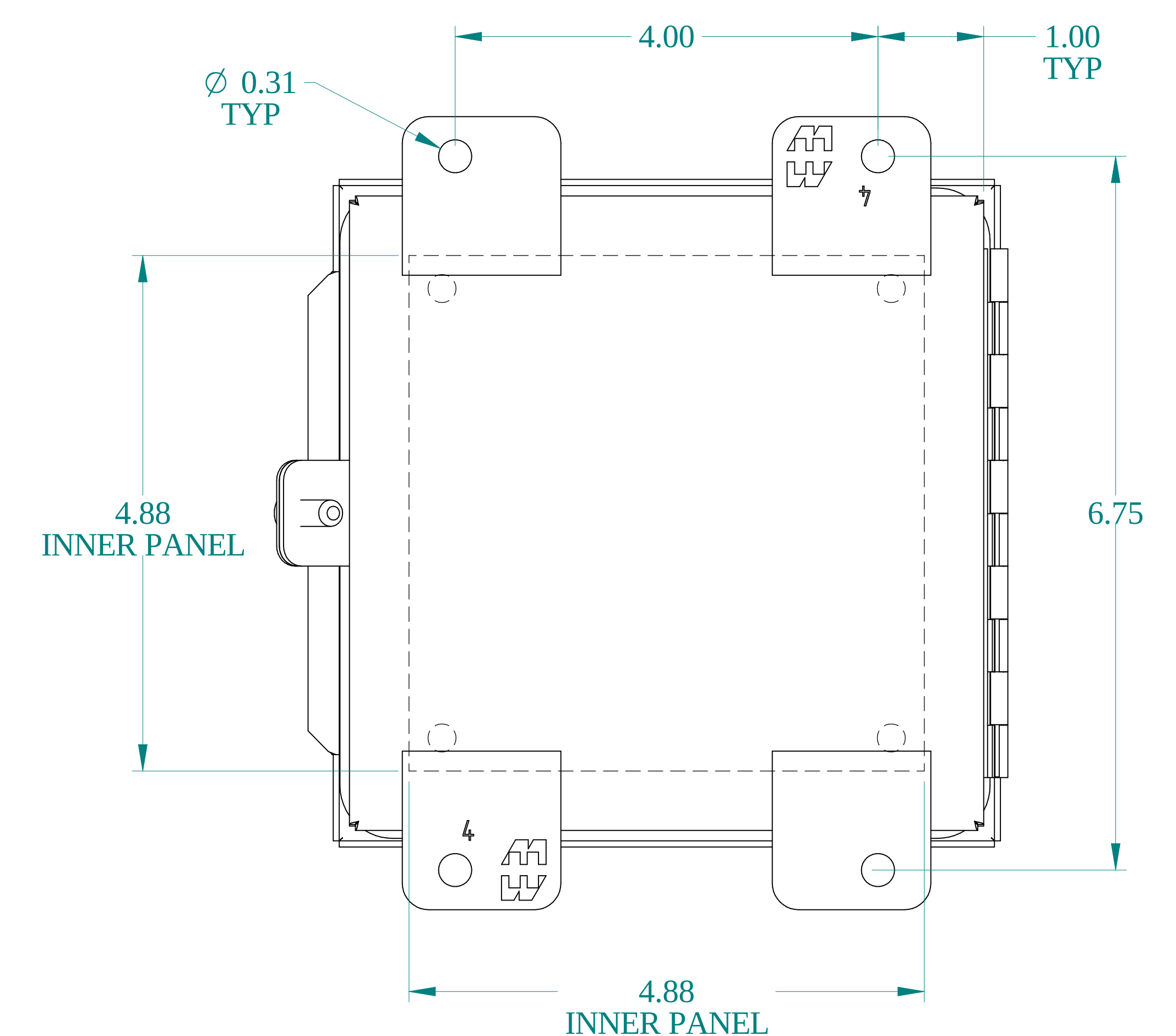
BACK VIEW
