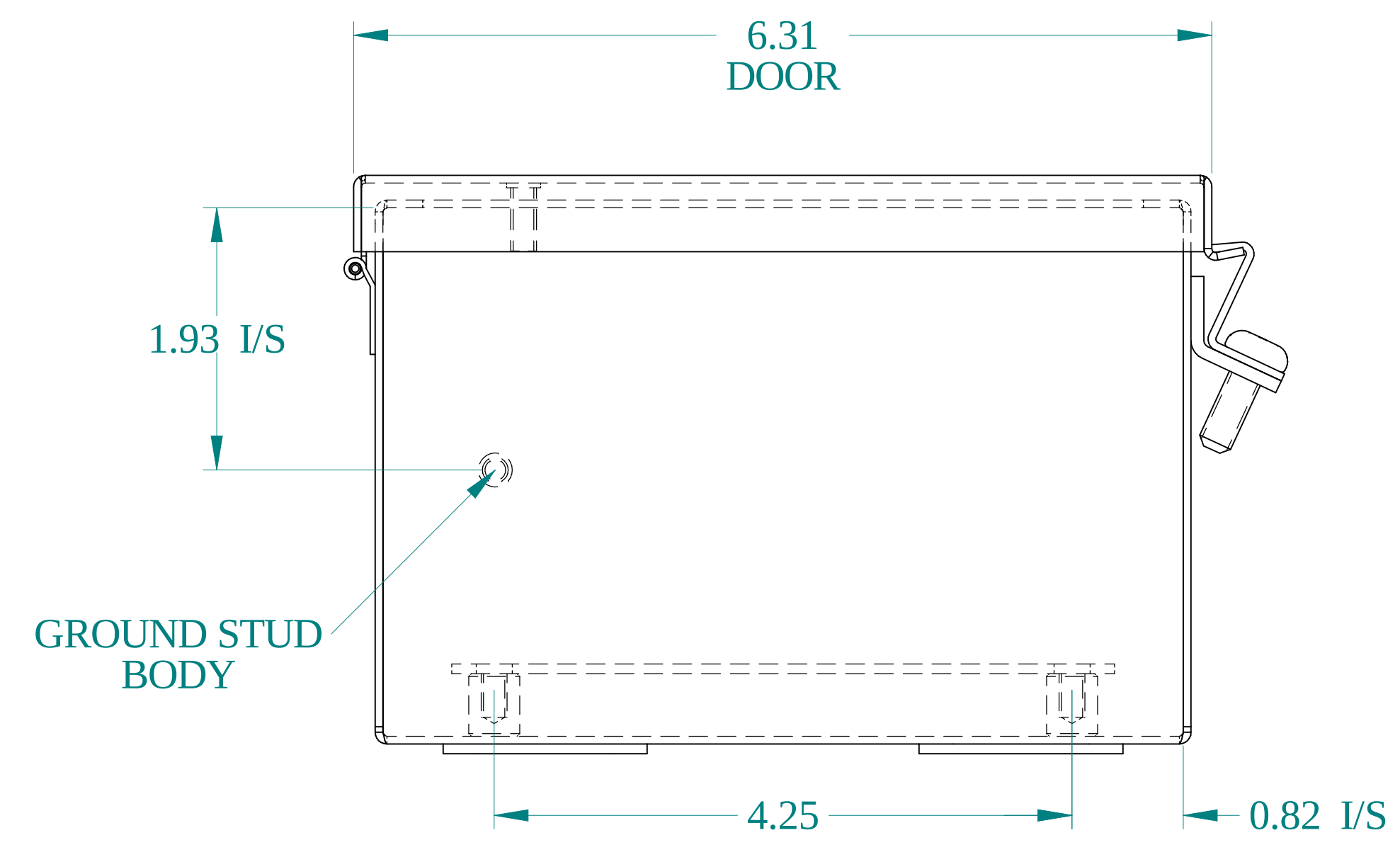
BOTTOM VIEW
