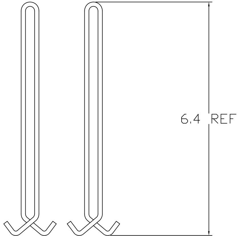
MAT'L .120 DIA. SAE #1010 STEEL WIRE FINISH: BRIGHT (ZINC OR CAD.)
