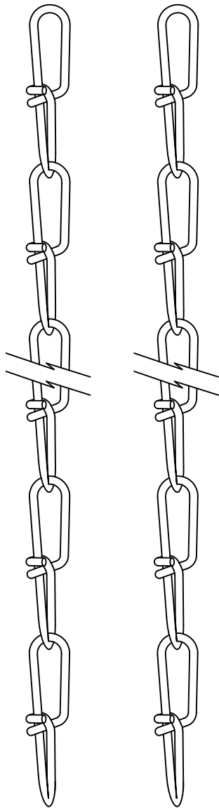
MAT'L .090 DIA. DOUBLE LOOP CHAIN FINISH: BRIGHT ZINC
