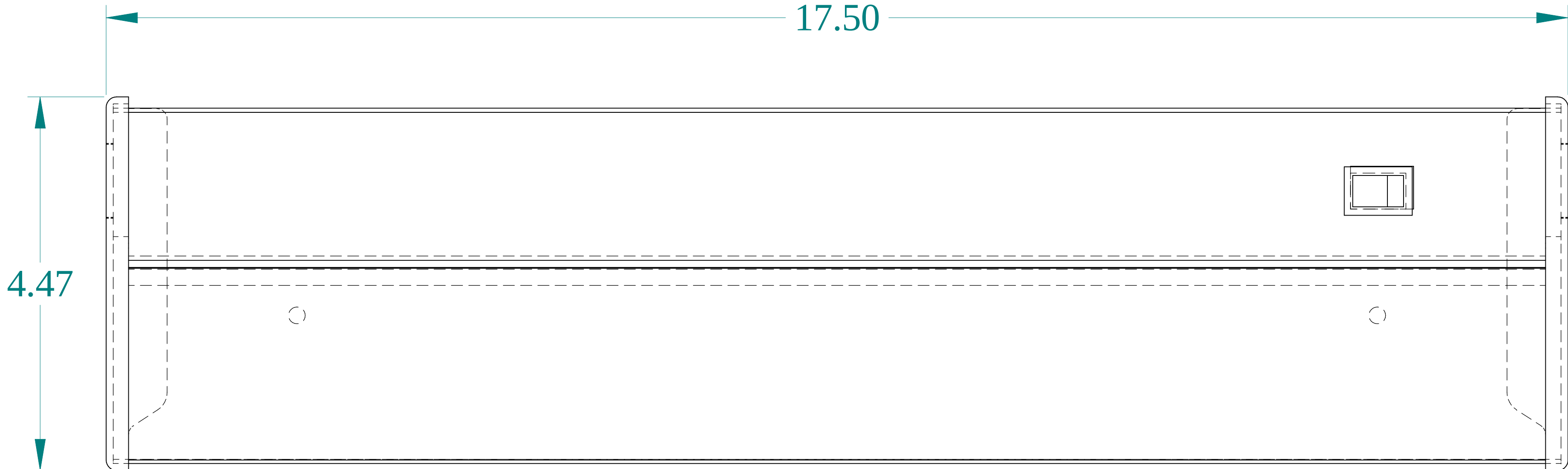
FRONT VIEW
