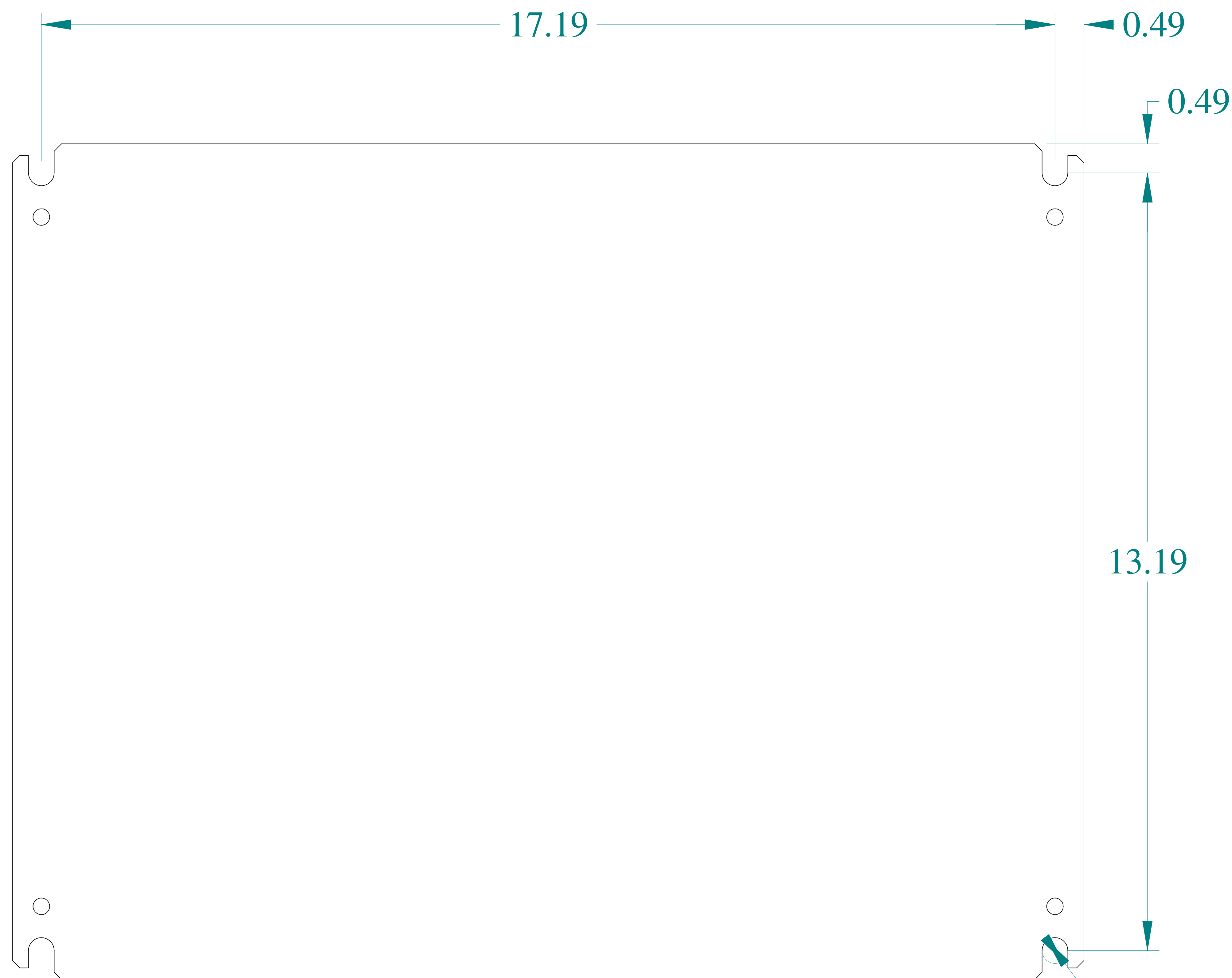
FRONT VIEW
