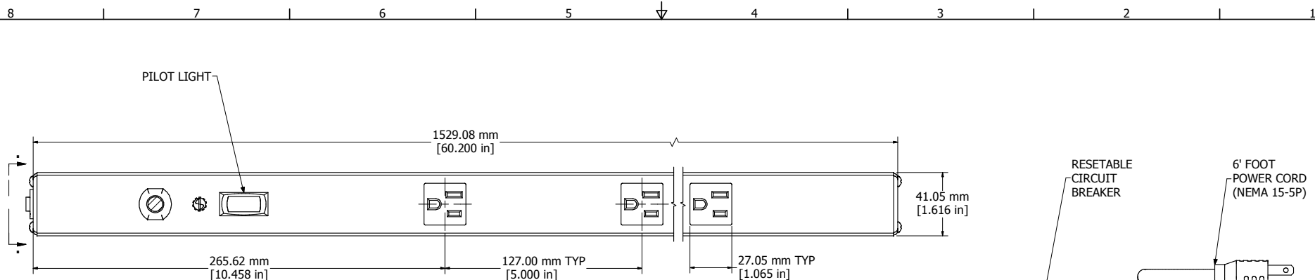
SECTION A-A (VIEW FROM FRONT)
