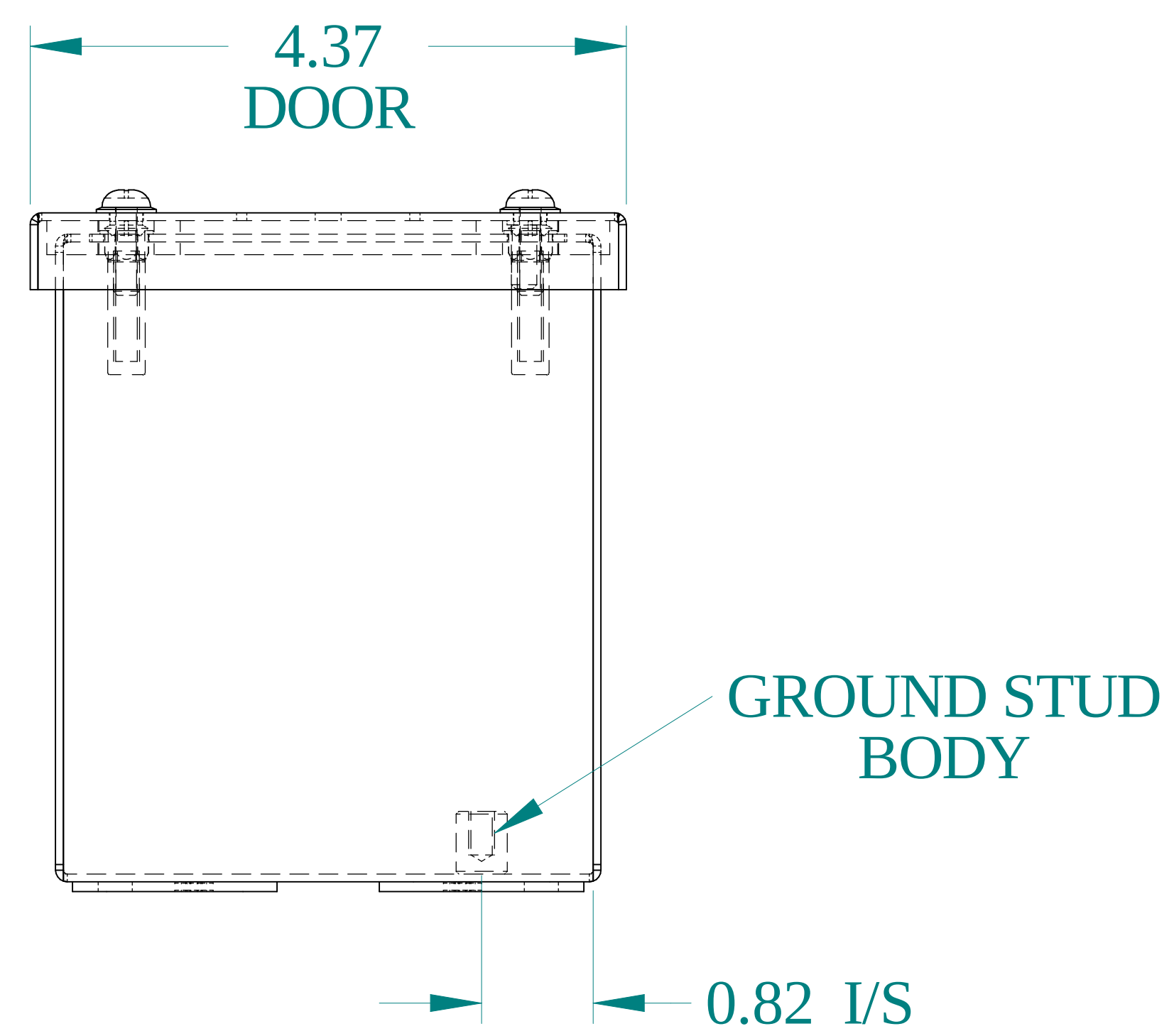
BOTTOM VIEW
