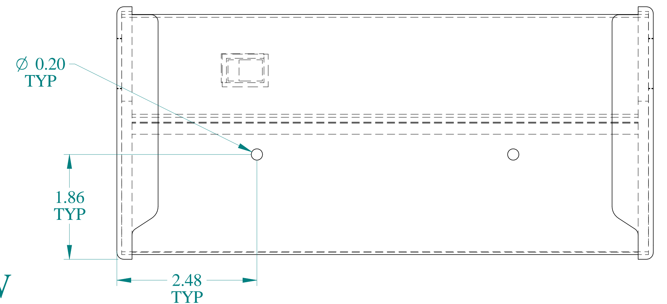
BACK VIEW
