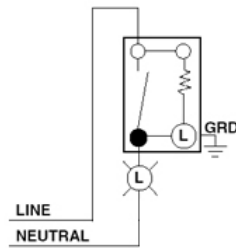
Wiring Diagram Single-Pole Lighted
