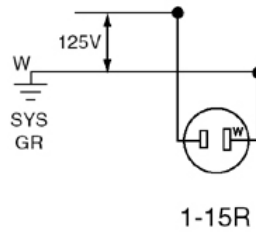
Wiring Diagram
