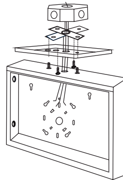
Ceiling Mount
