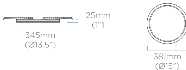
15" Die-cast Aluminum Round
