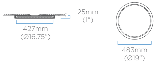
19" Die-cast Aluminum Round
