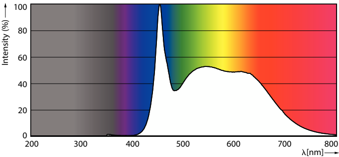
Spectral Power Distribution Colour - 8A19/LED/950/FR/Glass/E26/DIM 1FB T20
