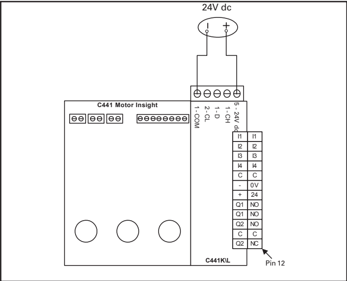
Figure 1. C441KL com module Wiring with C441
