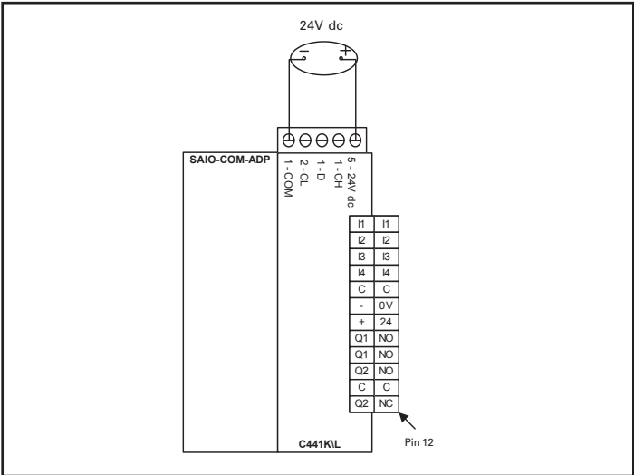
Figure 3. C441KL com module Wiring as Stand-alone I/O
