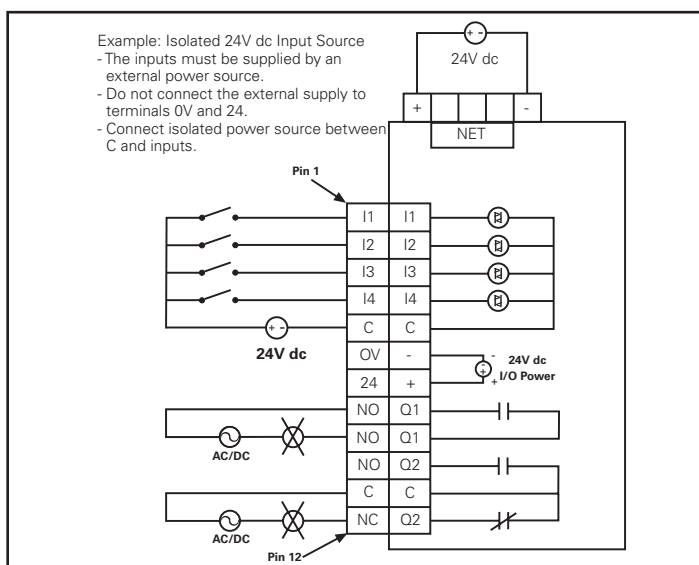
Figure 2. C441L 24V dc input Specification - Isolated
