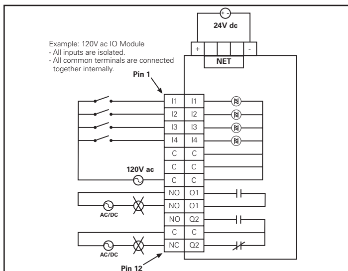
Figure 1. C441K—120 Vac Input Specification
