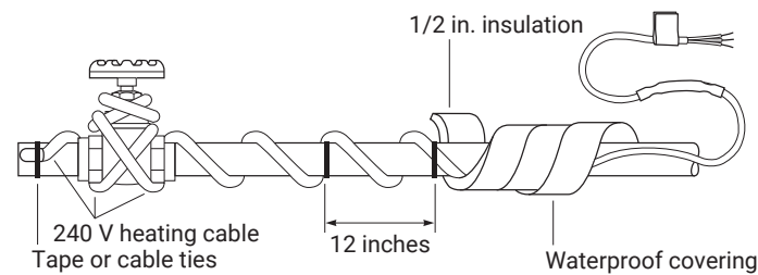
Spiral-traced Installation
