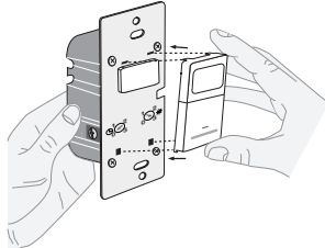
Attach new face by inserting bottom hinge tabs, then pivot and snap the color kit to attach
