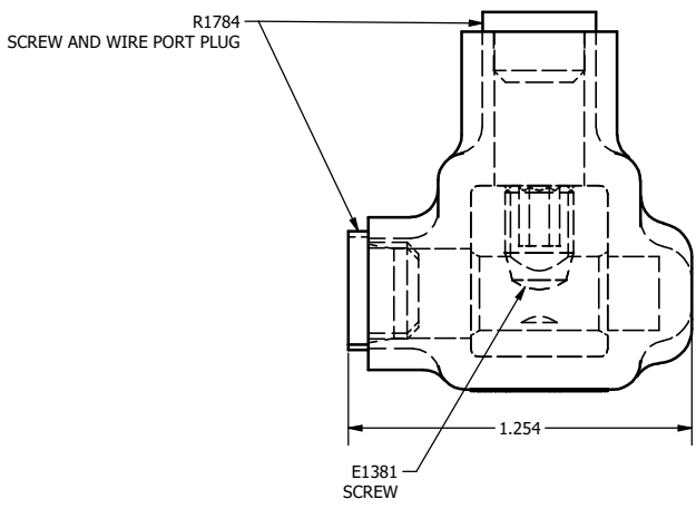
VIEW A-A SCALE 2.5:1
