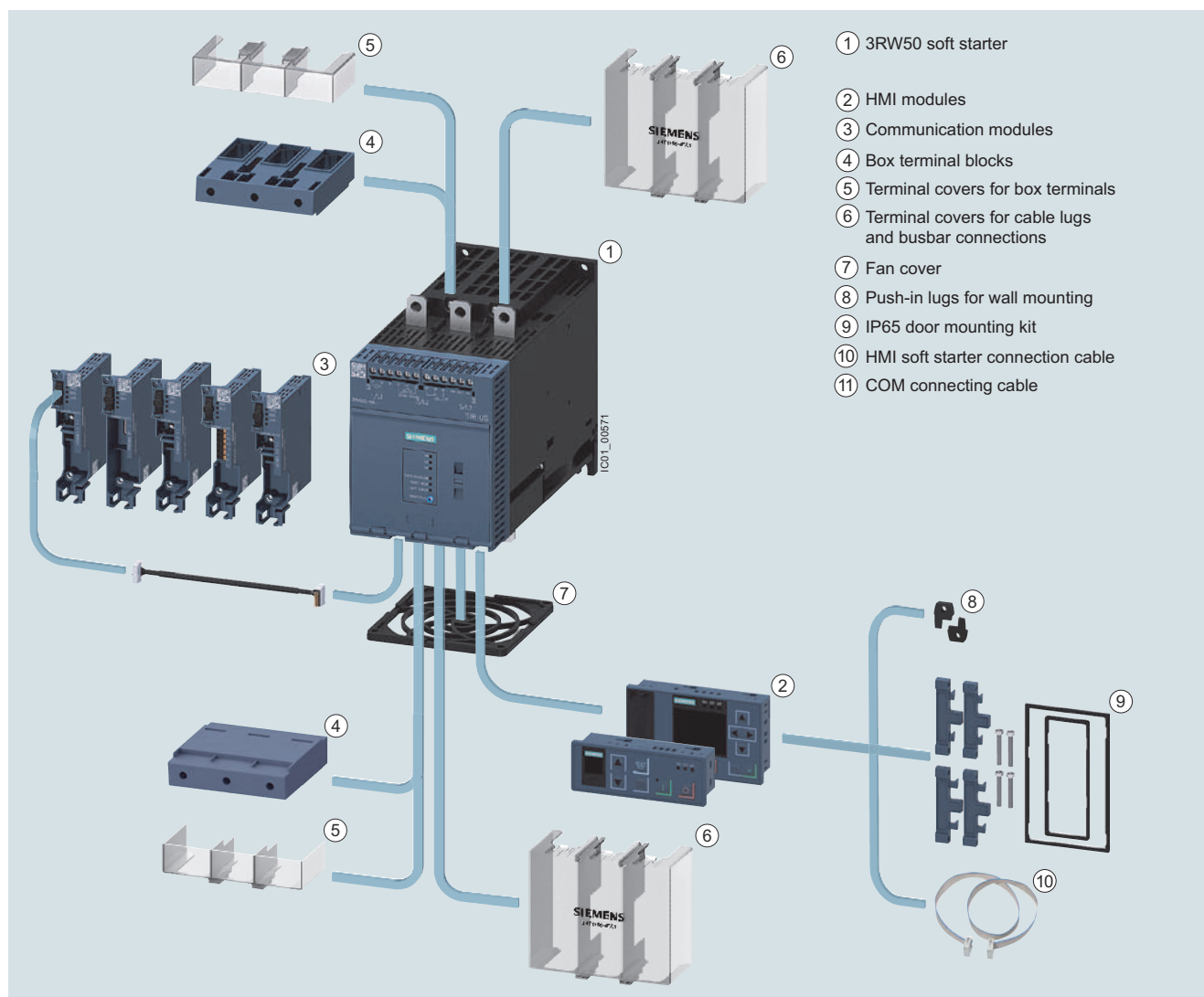
3RW50 Basic Performance soft starters with accessories (see page 17-261), for expansion with HMI module or communication module
