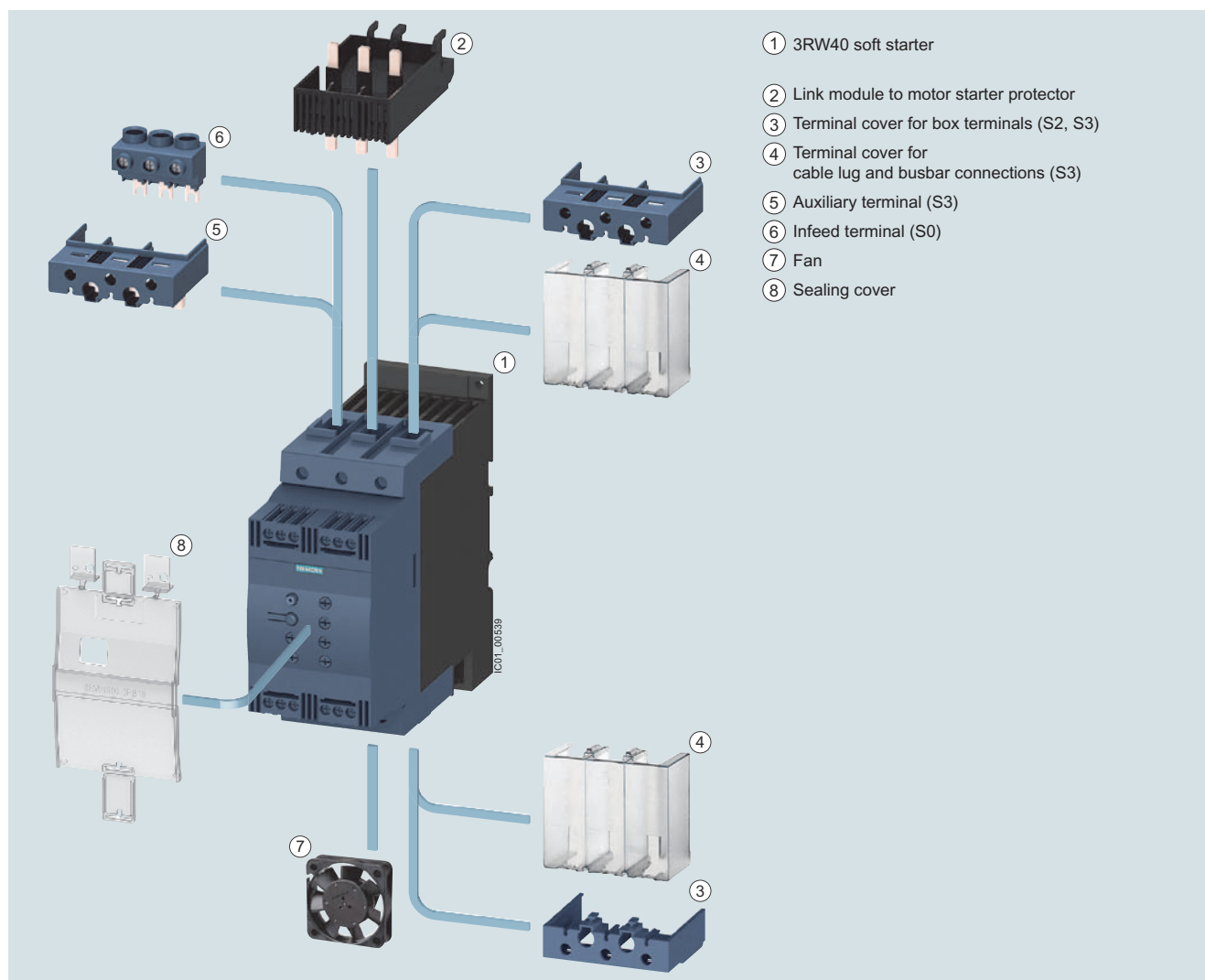
3RW40 Basic Performance soft starters with accessories (see page 17-272)
