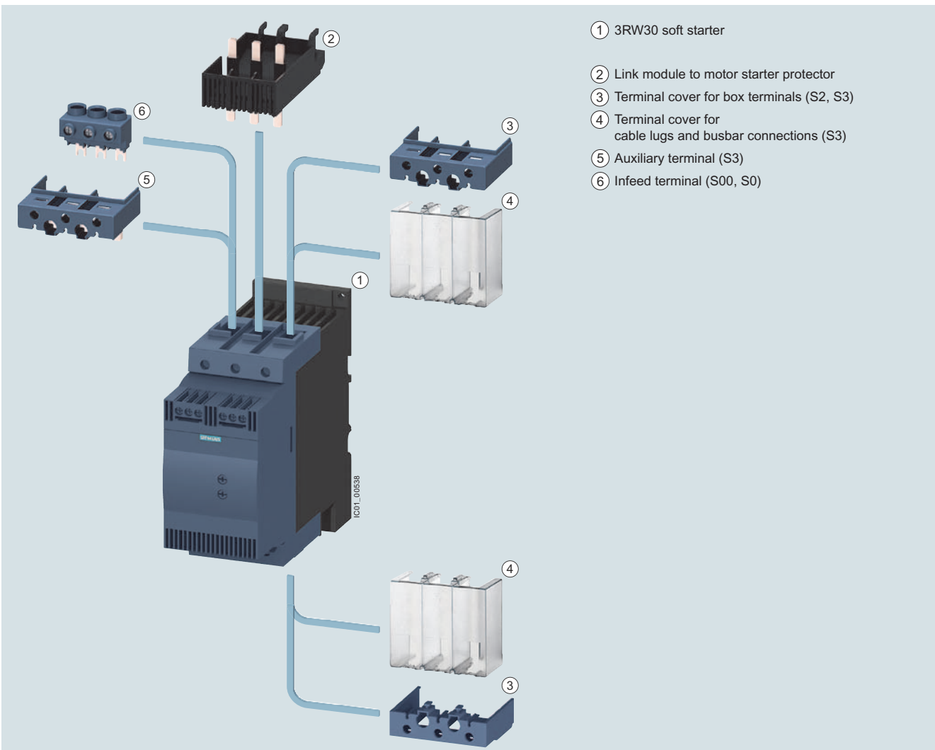
3RW30 Basic Performance soft starters with accessories (see page 17-283)
