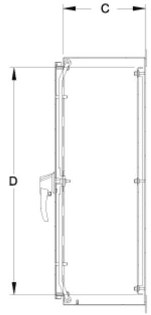
Section Y-Y
