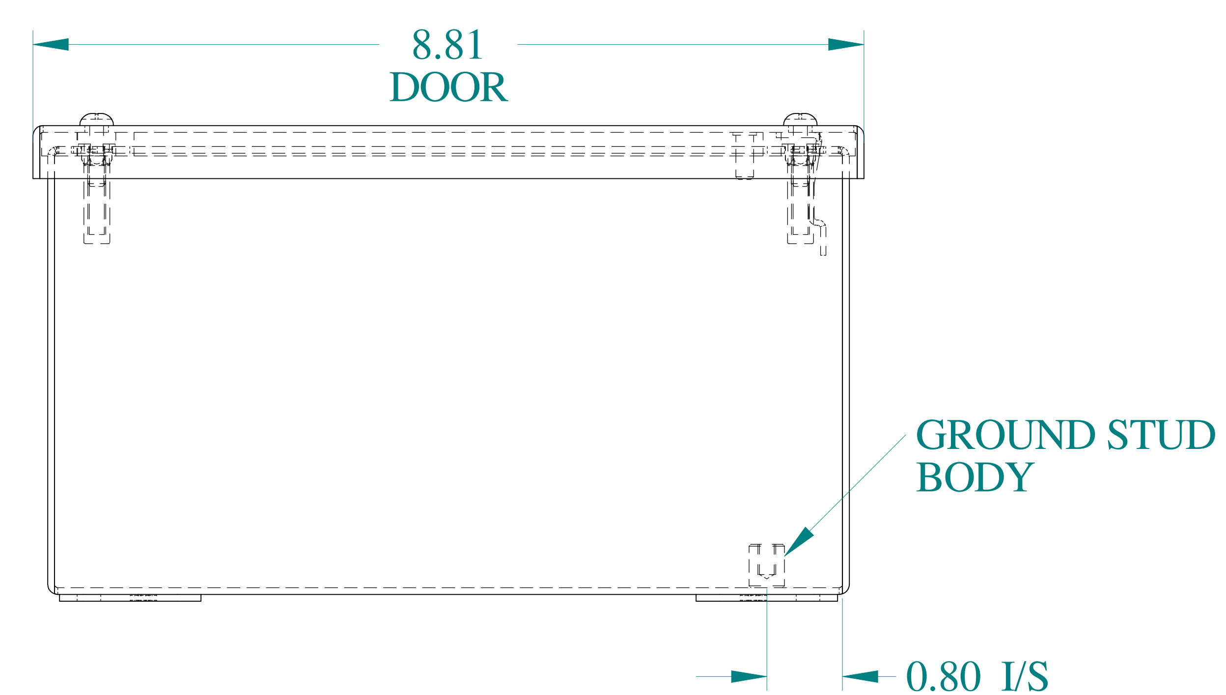
BOTTOM VIEW
