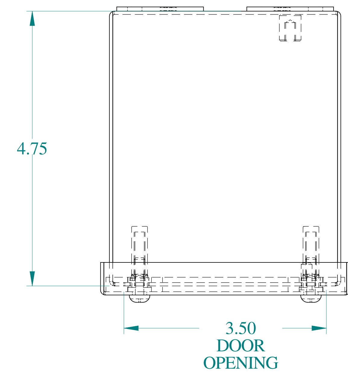
TOP VIEW
