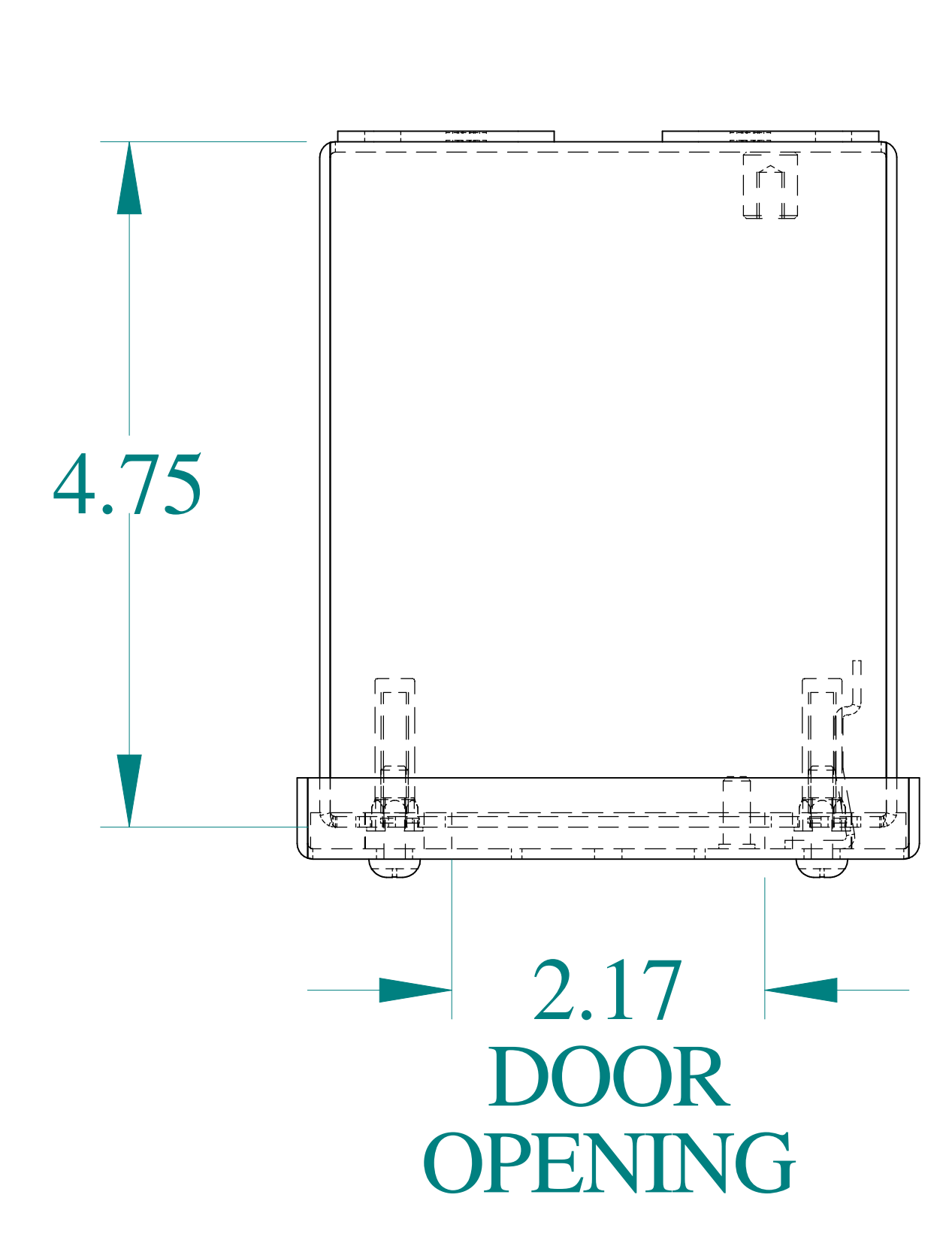
TOP VIEW
