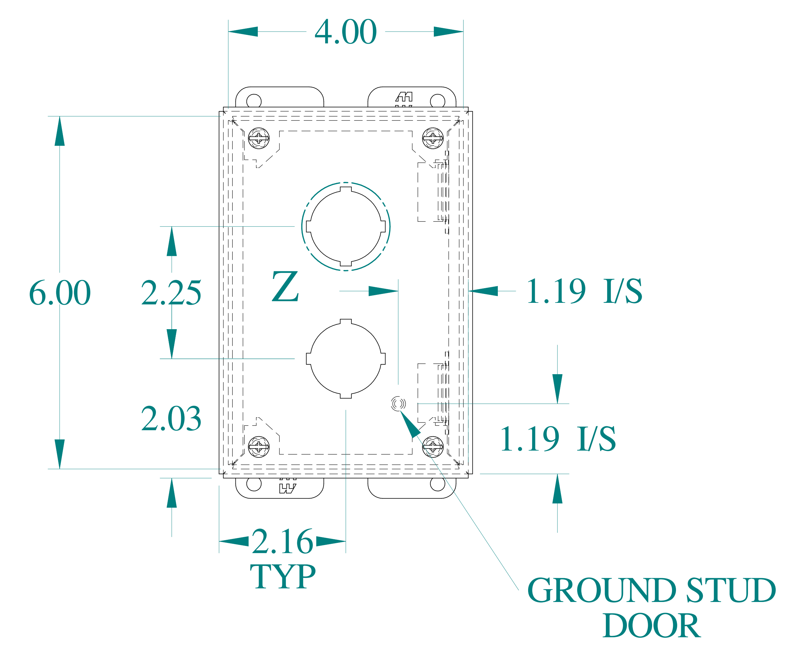
FRONT VIEW
