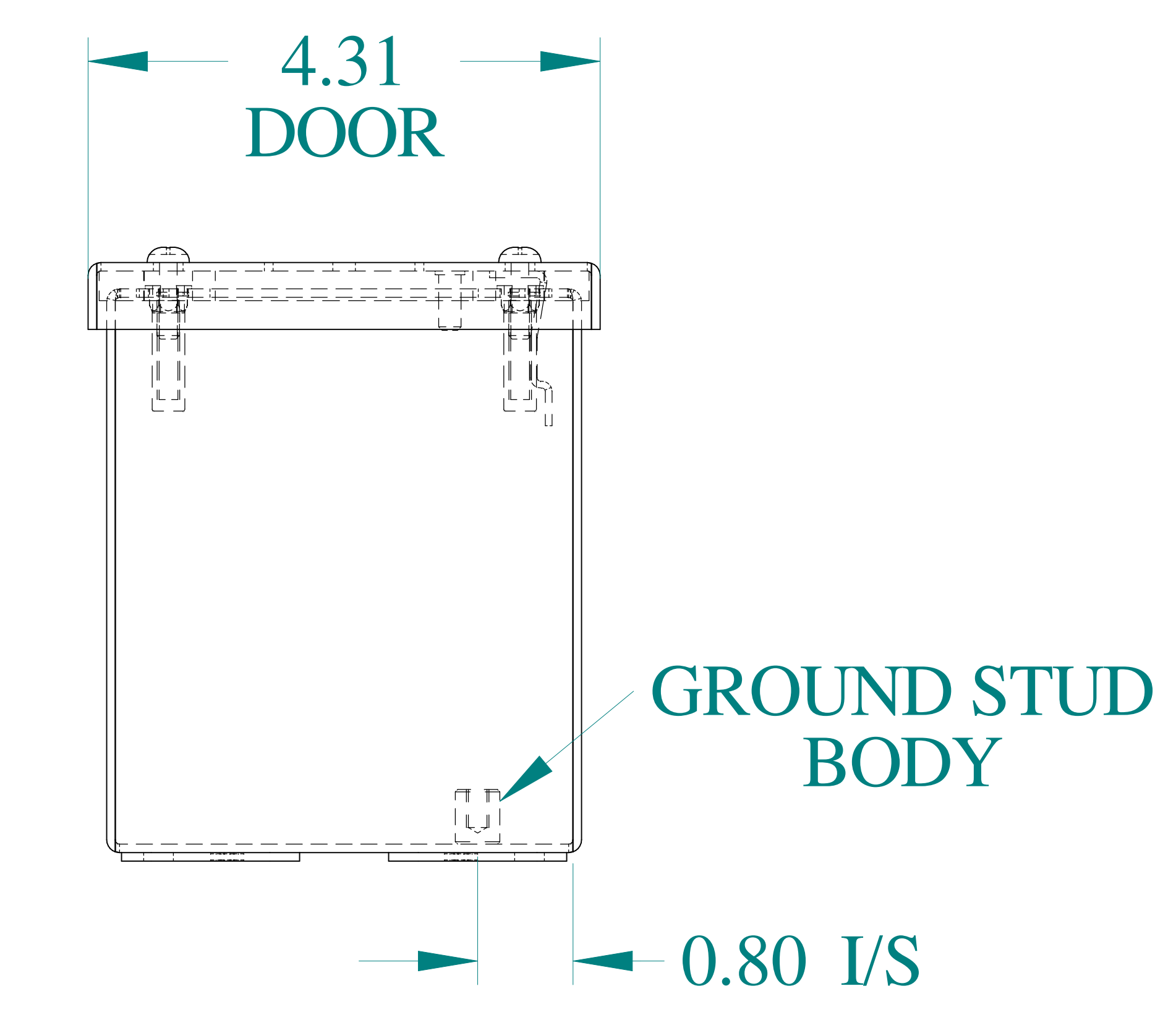
BOTTOM VIEW
