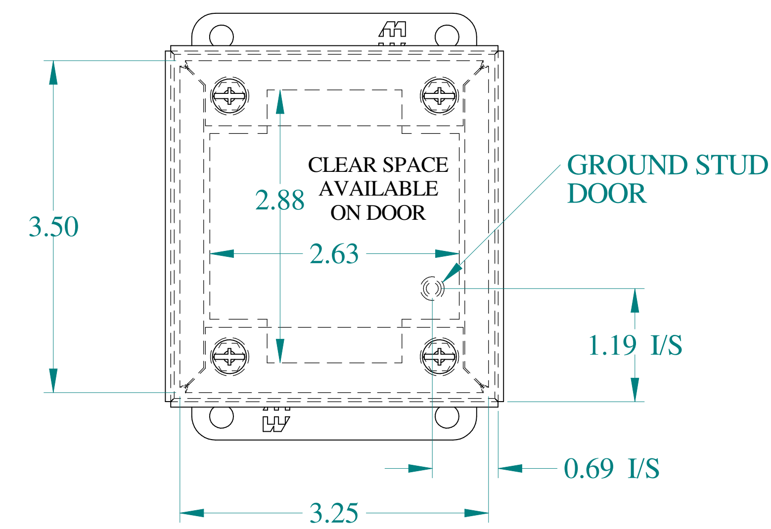
FRONT VIEW
