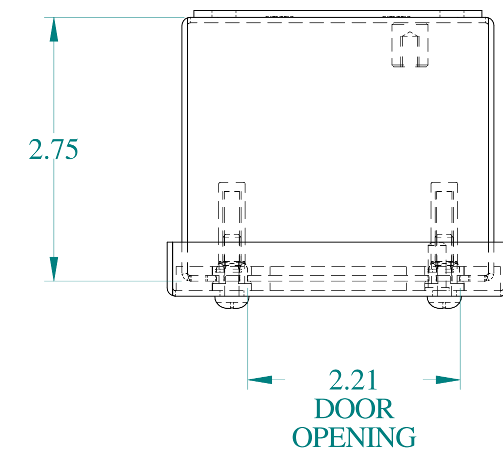
TOP VIEW
