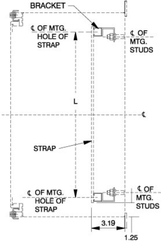
Side View
