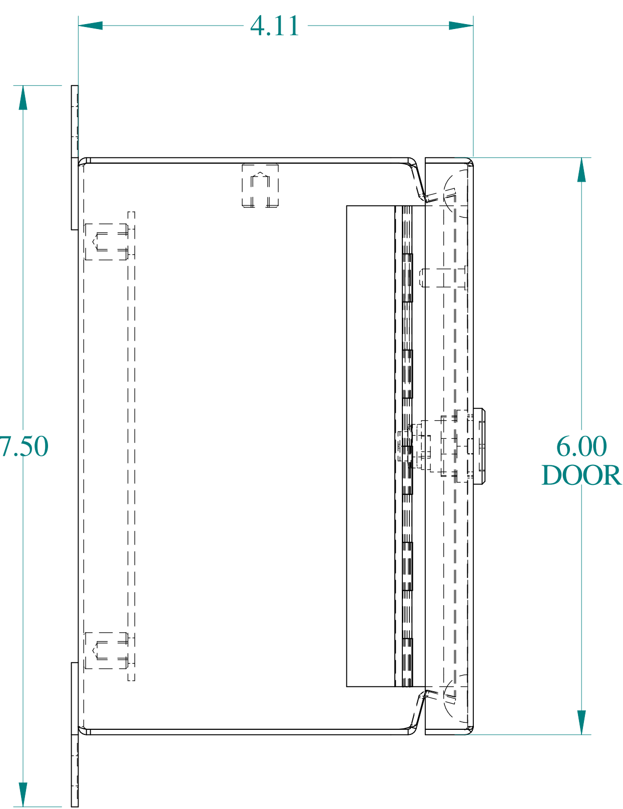
SIDE VIEW
