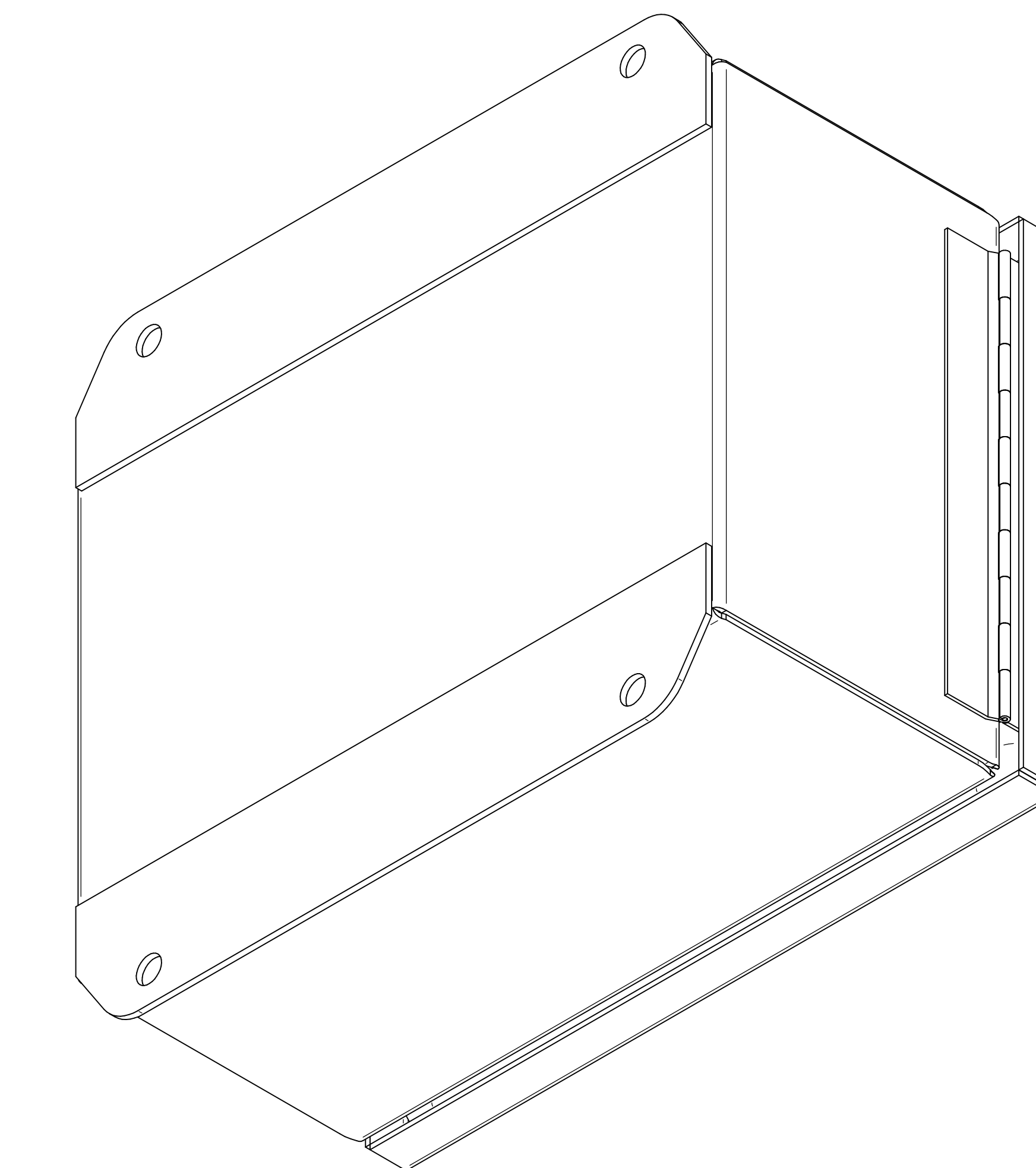
ISOMETRIC VIEWS
