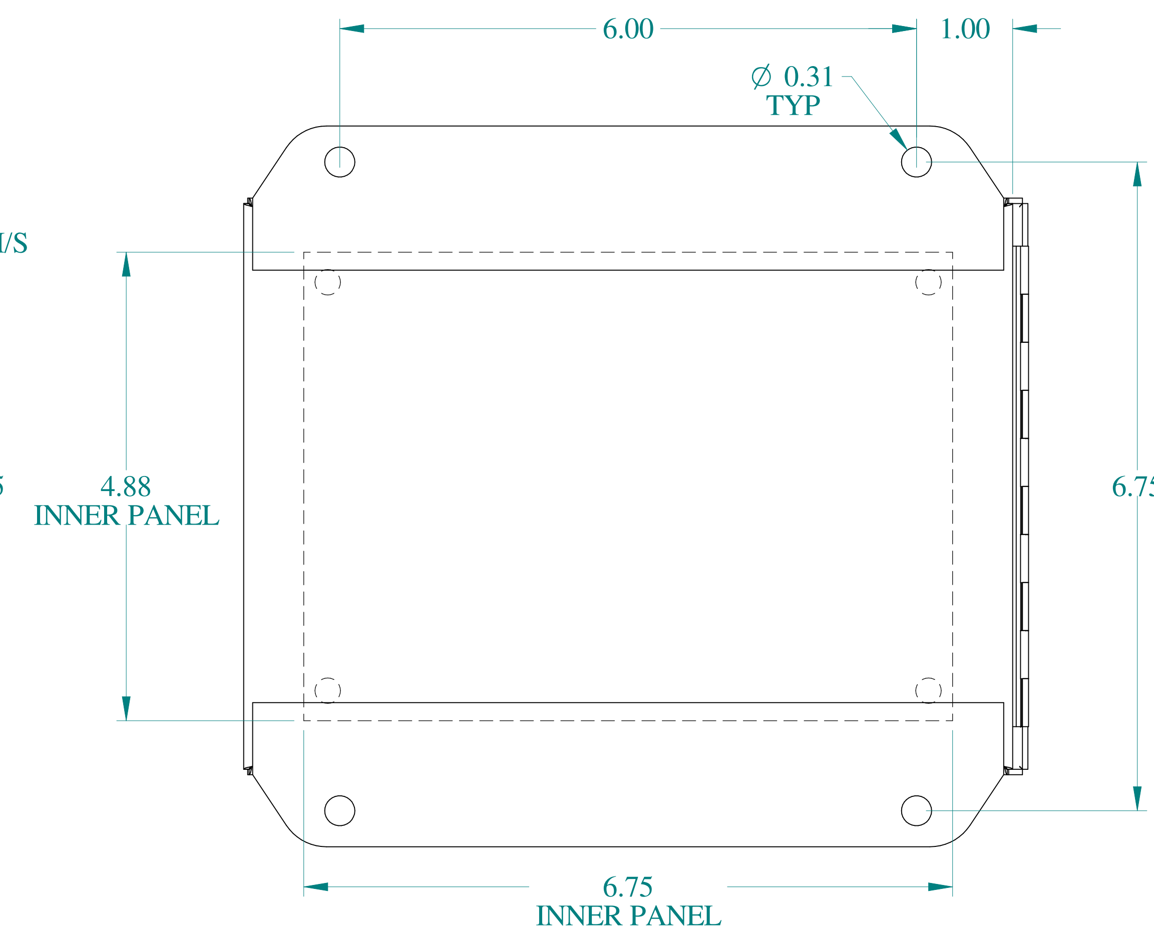
BACK VIEW
