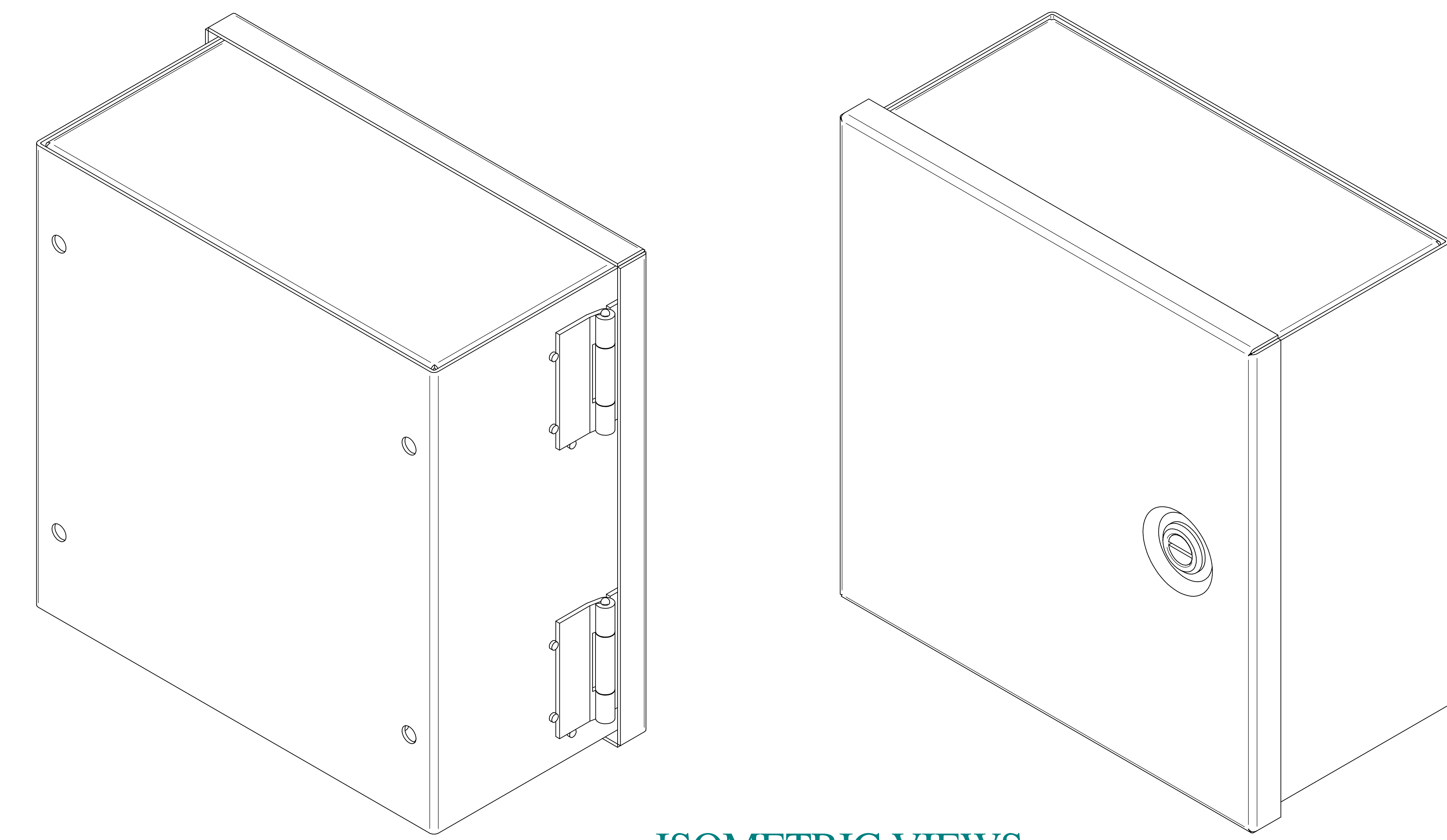
ISOMETRIC VIEWS
