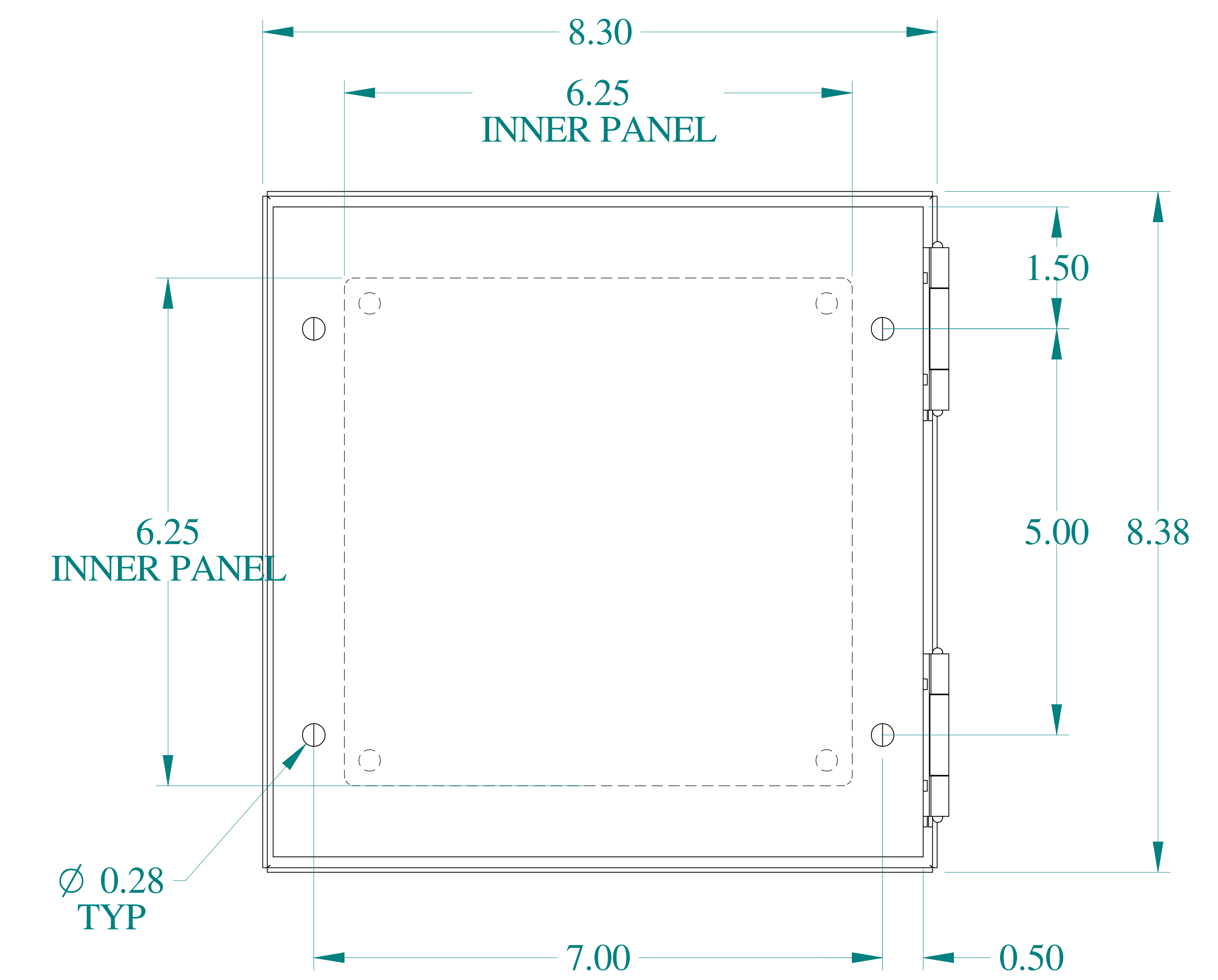
BACK VIEW
