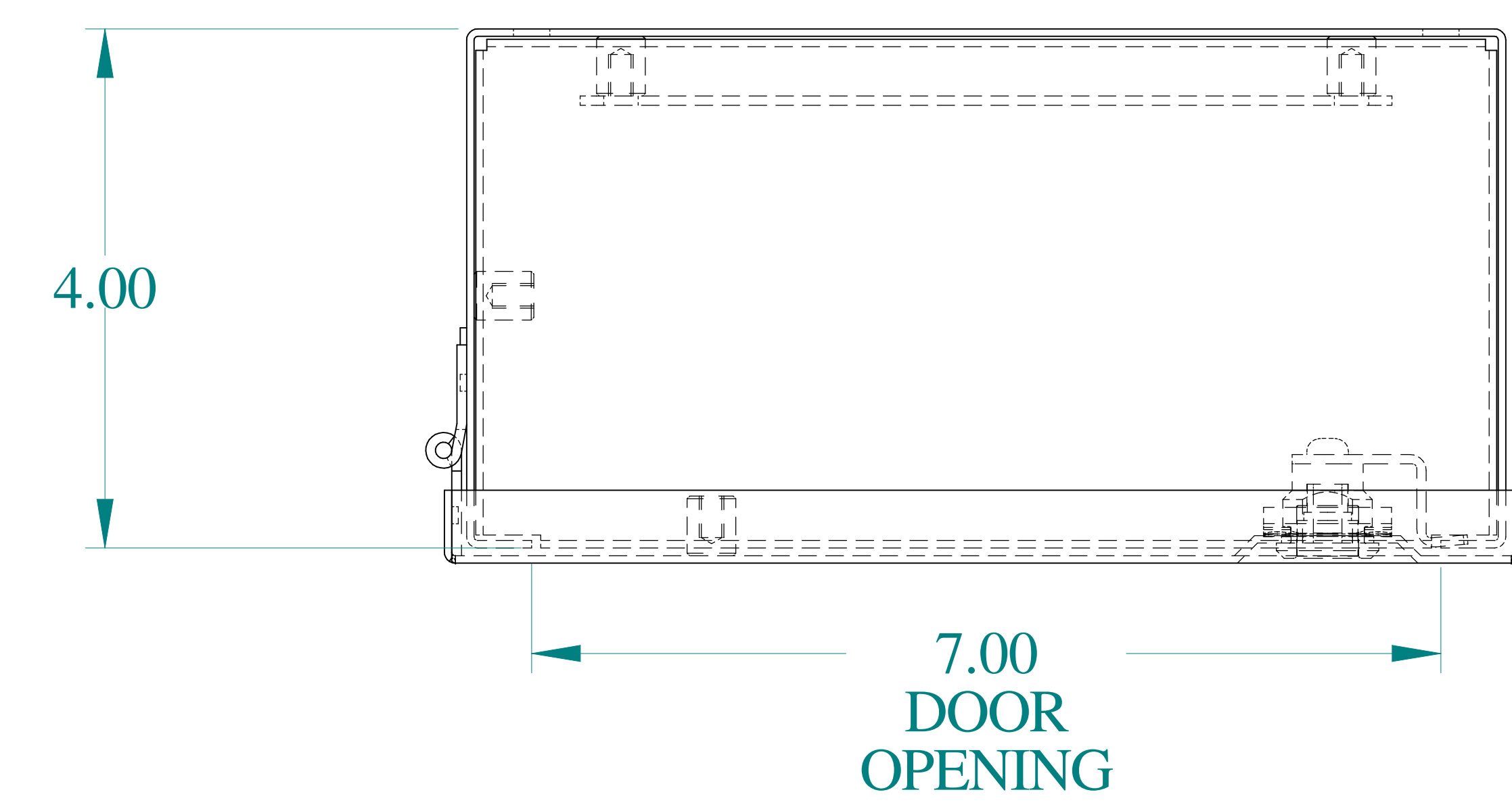
TOP VIEW
