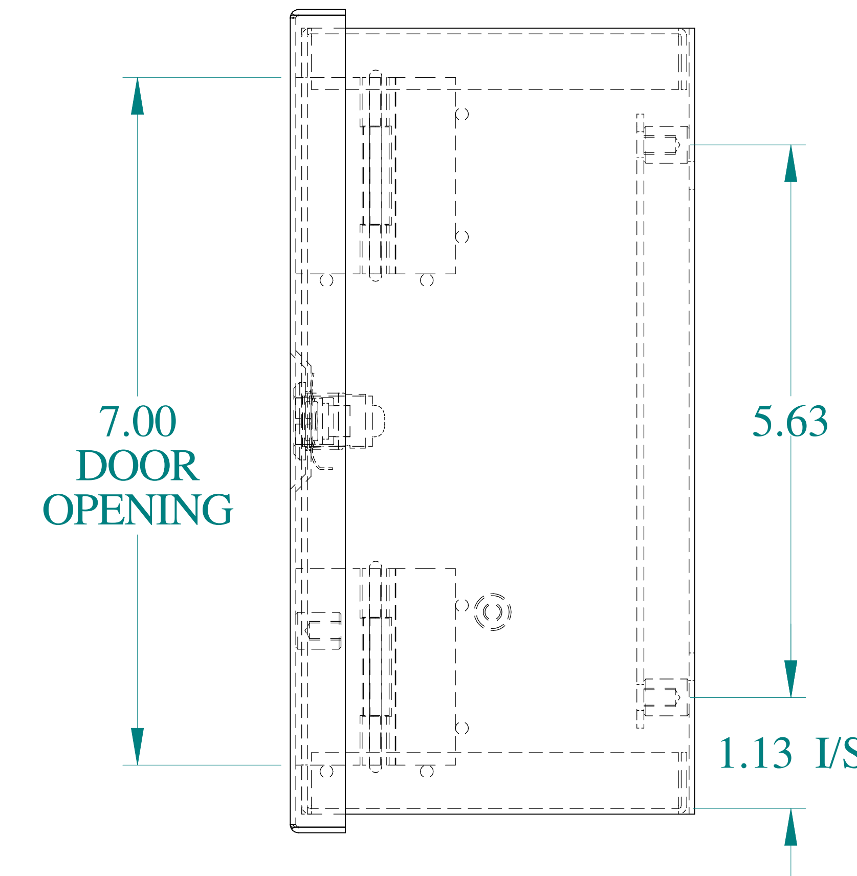
SIDE VIEW
