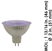
MR16 (GU5.3)
