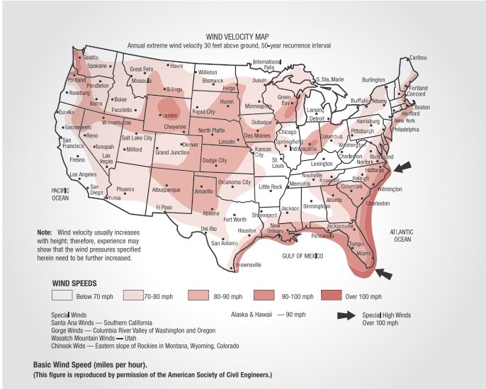
Figure 250-1USA and 250-2USA loading for grades B, C and D
