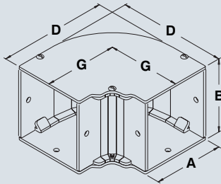
Elbow 90 degrees
