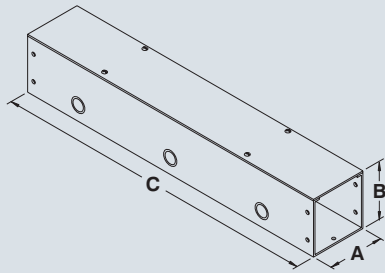
Straight section
