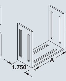
Joiner plate
