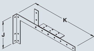
Drop hanger
