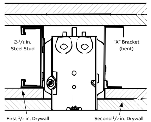
CI3004-LSSAX-1 Top View
