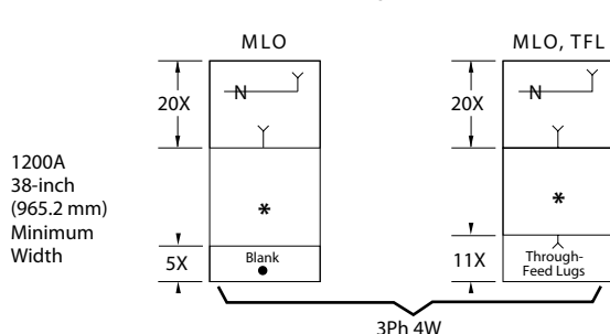
Figure 2-2. PRL4B Layout
