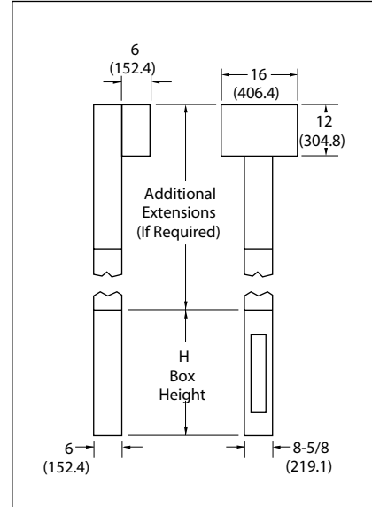
Figure 2.11 PRL2a-LX Trough Extension, Dimensions in Inches(mm)
