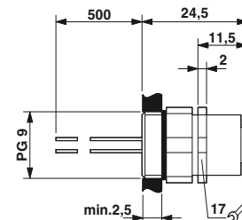
Dimensions: socket, can be positioned
