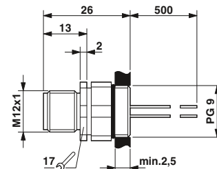
Dimensions: plug, can be positioned
