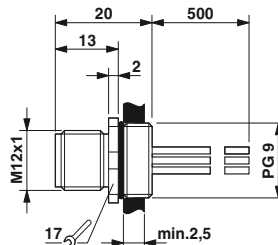
Dimensions: plug
