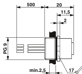
Dimensions: socket
